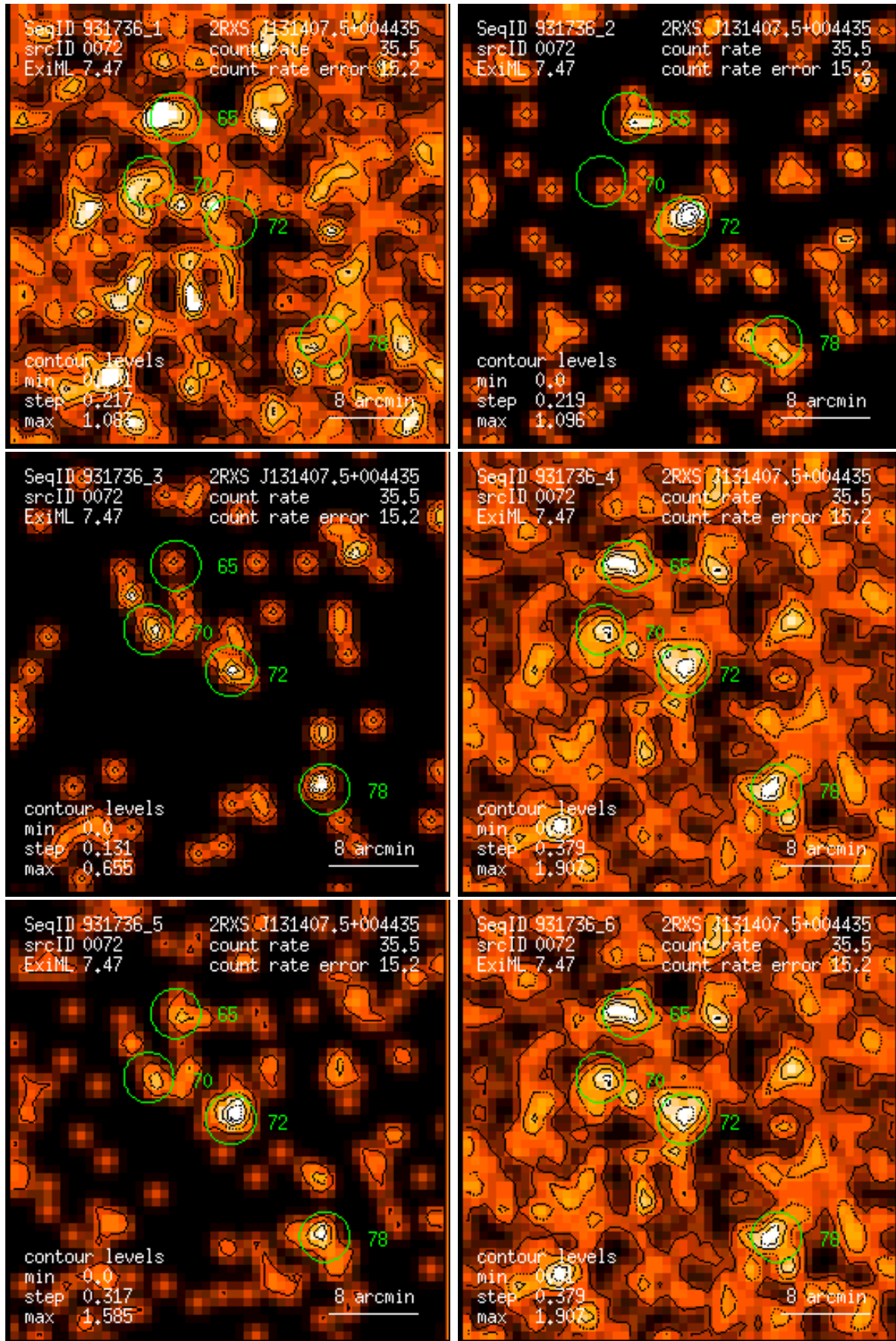
Figure 72: RASS 931736: detection 0072: band rate images, Gaussian filter: (1) PSPC channels 11 – 41, (2) 52 – 90, (3) 91 – 201, (4) 11 – 235, (5) 52 – 201, (6) 11 – 201. Broad band rates in counts/ks. Band rate contour levels in counts/ks/arcmin 2 .
