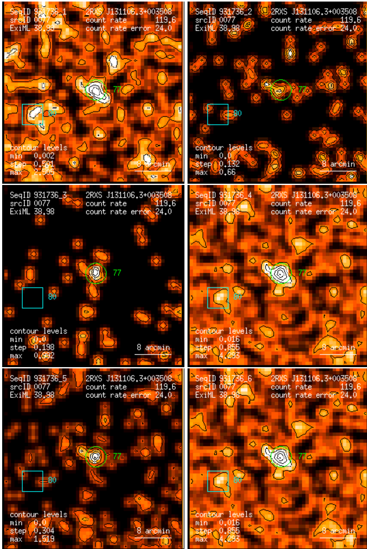
Figure 77: RASS 931736: detection 0077: band rate images, Gaussian filter: (1) PSPC channels 11 – 41, (2) 52 – 90, (3) 91 – 201, (4) 11 – 235, (5) 52 – 201, (6) 11 – 201. Broad band rates in counts/ks. Band rate contour levels in counts/ks/arcmin 2 .
