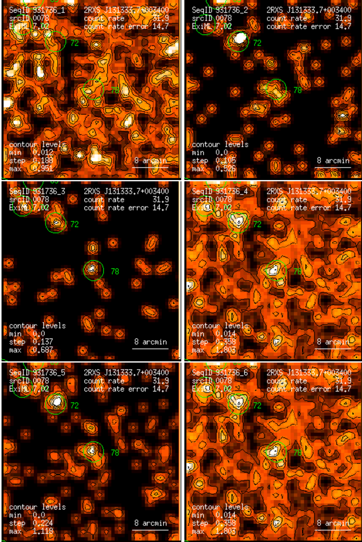
Figure 78: RASS 931736: detection 0078: band rate images, Gaussian filter: (1) PSPC channels 11 – 41, (2) 52 – 90, (3) 91 – 201, (4) 11 – 235, (5) 52 – 201, (6) 11 – 201. Broad band rates in counts/ks. Band rate contour levels in counts/ks/arcmin 2 .
