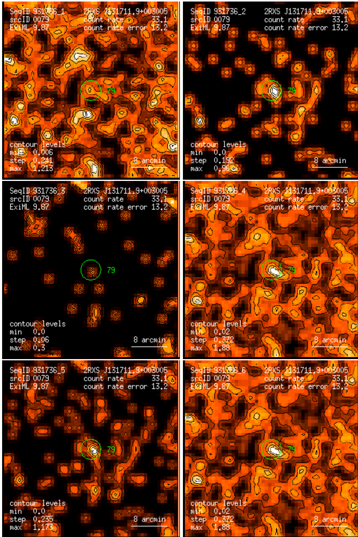
Figure 79: RASS 931736: detection 0079: band rate images, Gaussian filter: (1) PSPC channels 11 – 41, (2) 52 – 90, (3) 91 – 201, (4) 11 – 235, (5) 52 – 201, (6) 11 – 201. Broad band rates in counts/ks. Band rate contour levels in counts/ks/arcmin 2 .
