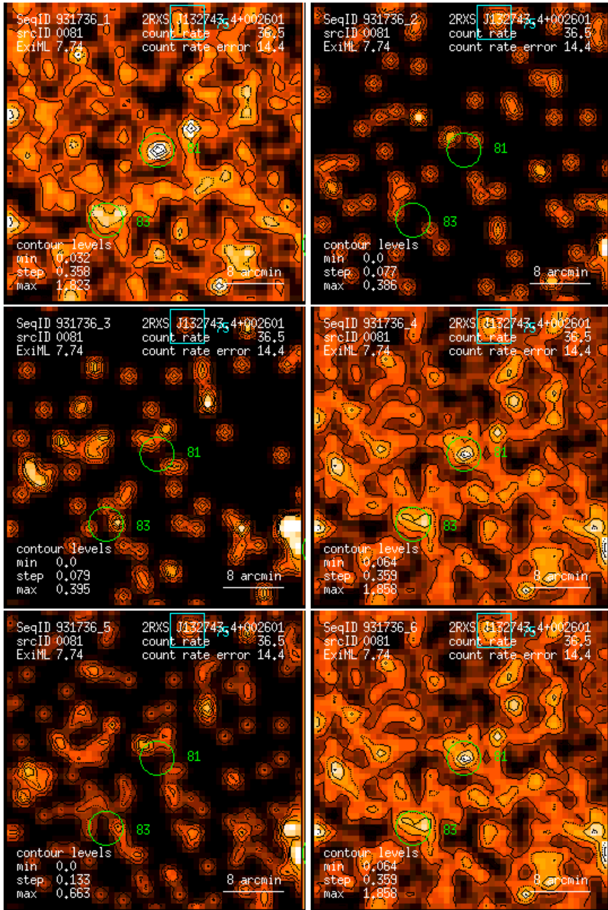
Figure 81: RASS 931736: detection 0081: band rate images, Gaussian filter: (1) PSPC channels 11 – 41, (2) 52 – 90, (3) 91 – 201, (4) 11 – 235, (5) 52 – 201, (6) 11 – 201. Broad band rates in counts/ks. Band rate contour levels in counts/ks/arcmin 2 .
