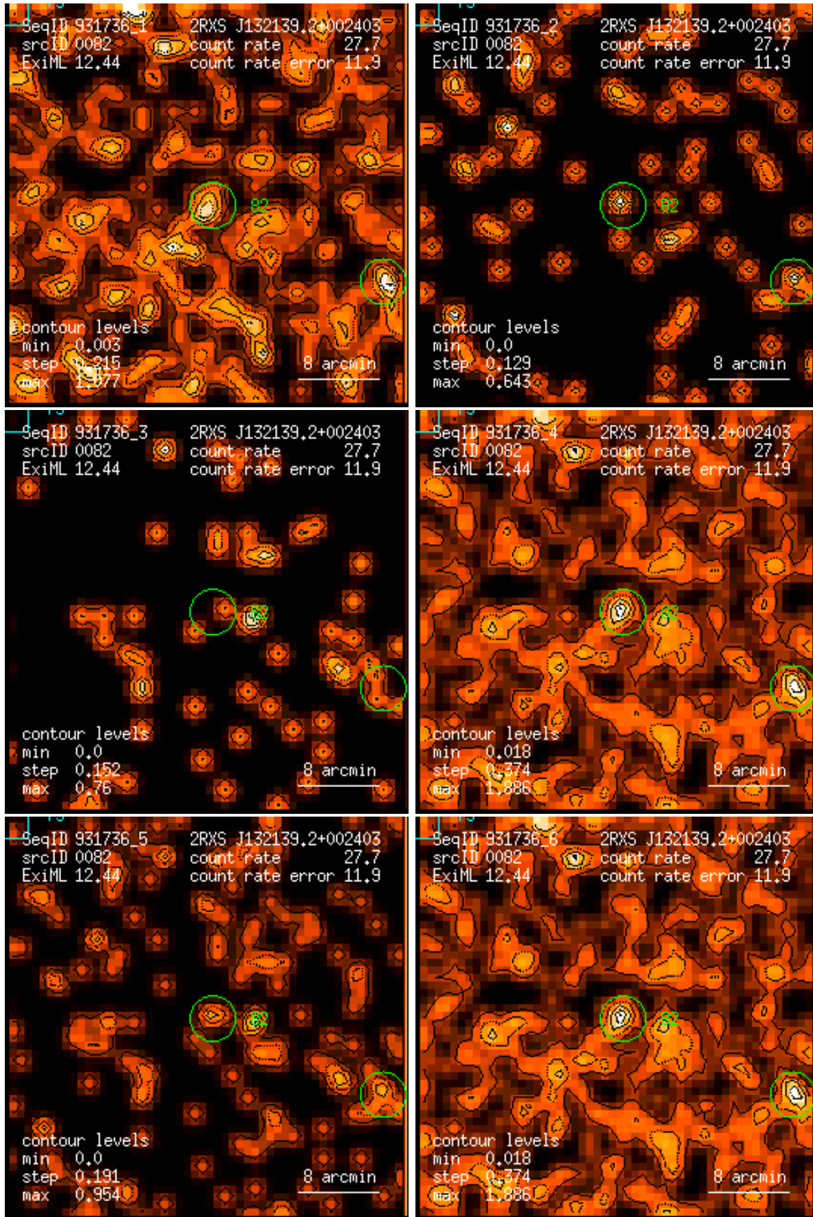
Figure 82: RASS 931736: detection 0082: band rate images, Gaussian filter: (1) PSPC channels 11 – 41, (2) 52 – 90, (3) 91 – 201, (4) 11 – 235, (5) 52 – 201, (6) 11 – 201. Broad band rates in counts/ks. Band rate contour levels in counts/ks/arcmin 2 .
