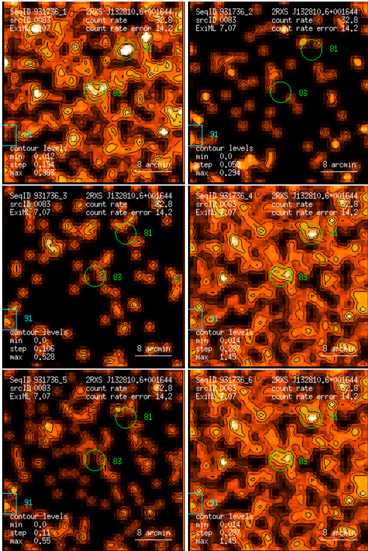
Figure 83: RASS 931736: detection 0083: band rate images, Gaussian filter: (1) PSPC channels 11 – 41, (2) 52 – 90, (3) 91 – 201, (4) 11 – 235, (5) 52 – 201, (6) 11 – 201. Broad band rates in counts/ks. Band rate contour levels in counts/ks/arcmin 2 .
