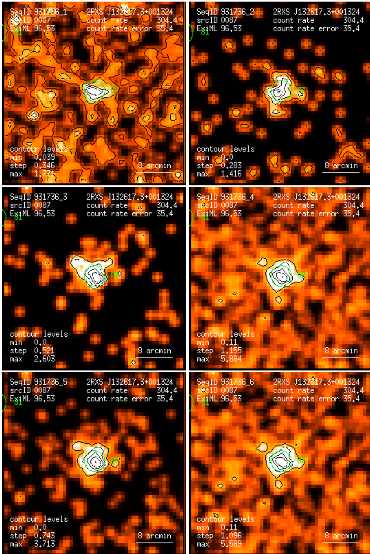
Figure 87: RASS 931736: detection 0087: band rate images, Gaussian filter: (1) PSPC channels 11 – 41, (2) 52 – 90, (3) 91 – 201, (4) 11 – 235, (5) 52 – 201, (6) 11 – 201. Broad band rates in counts/ks. Band rate contour levels in counts/ks/arcmin 2 .
