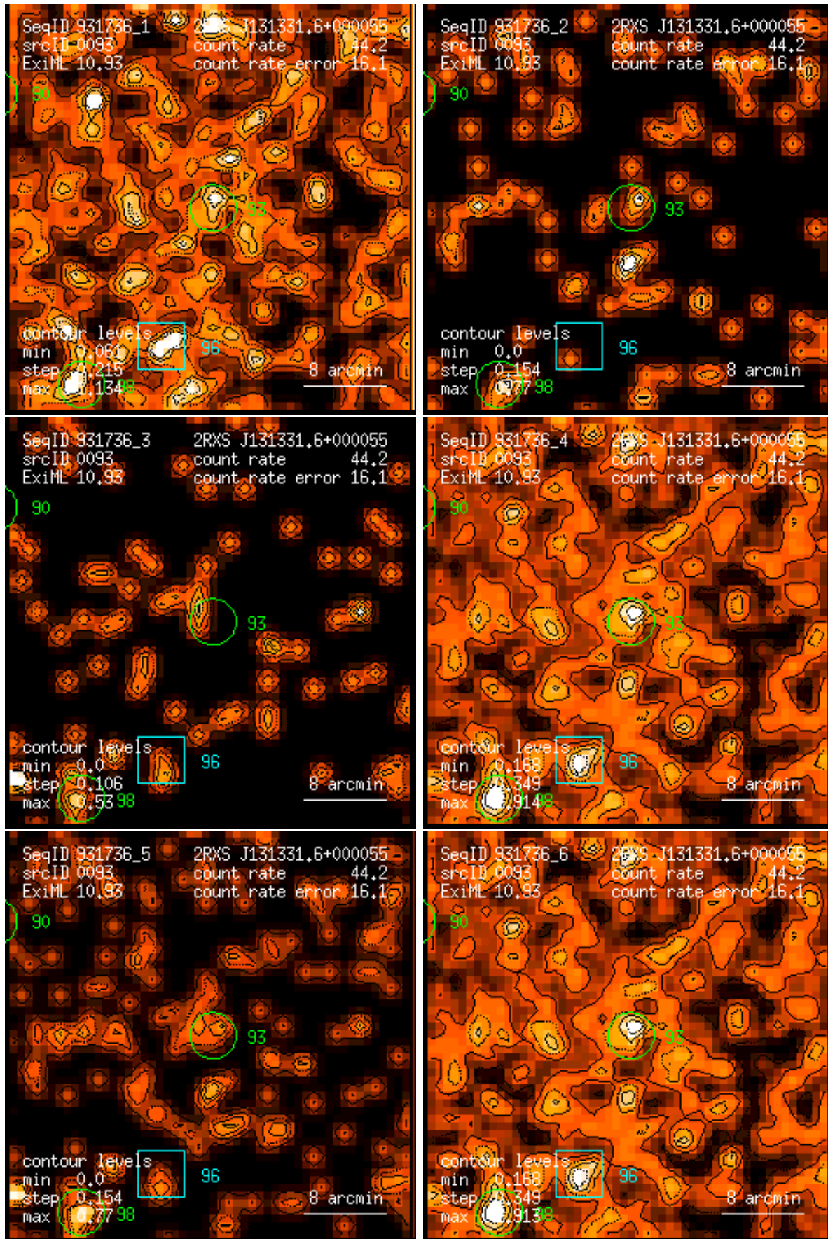
Figure 93: RASS 931736: detection 0093: band rate images, Gaussian filter: (1) PSPC channels 11 – 41, (2) 52 – 90, (3) 91 – 201, (4) 11 – 235, (5) 52 – 201, (6) 11 – 201. Broad band rates in counts/ks. Band rate contour levels in counts/ks/arcmin 2 .
