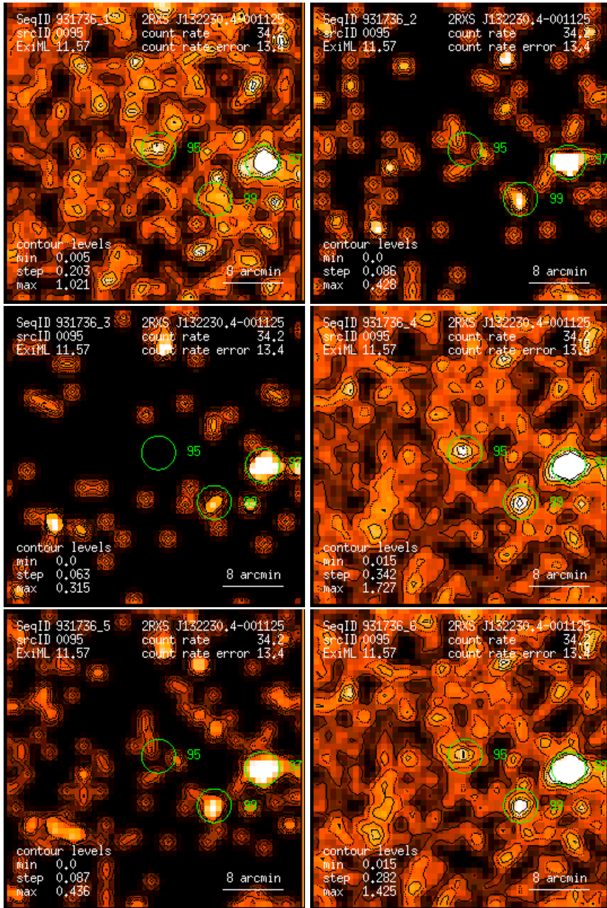
Figure 95: RASS 931736: detection 0095: band rate images, Gaussian filter: (1) PSPC channels 11 – 41, (2) 52 – 90, (3) 91 – 201, (4) 11 – 235, (5) 52 – 201, (6) 11 – 201. Broad band rates in counts/ks. Band rate contour levels in counts/ks/arcmin 2 .
