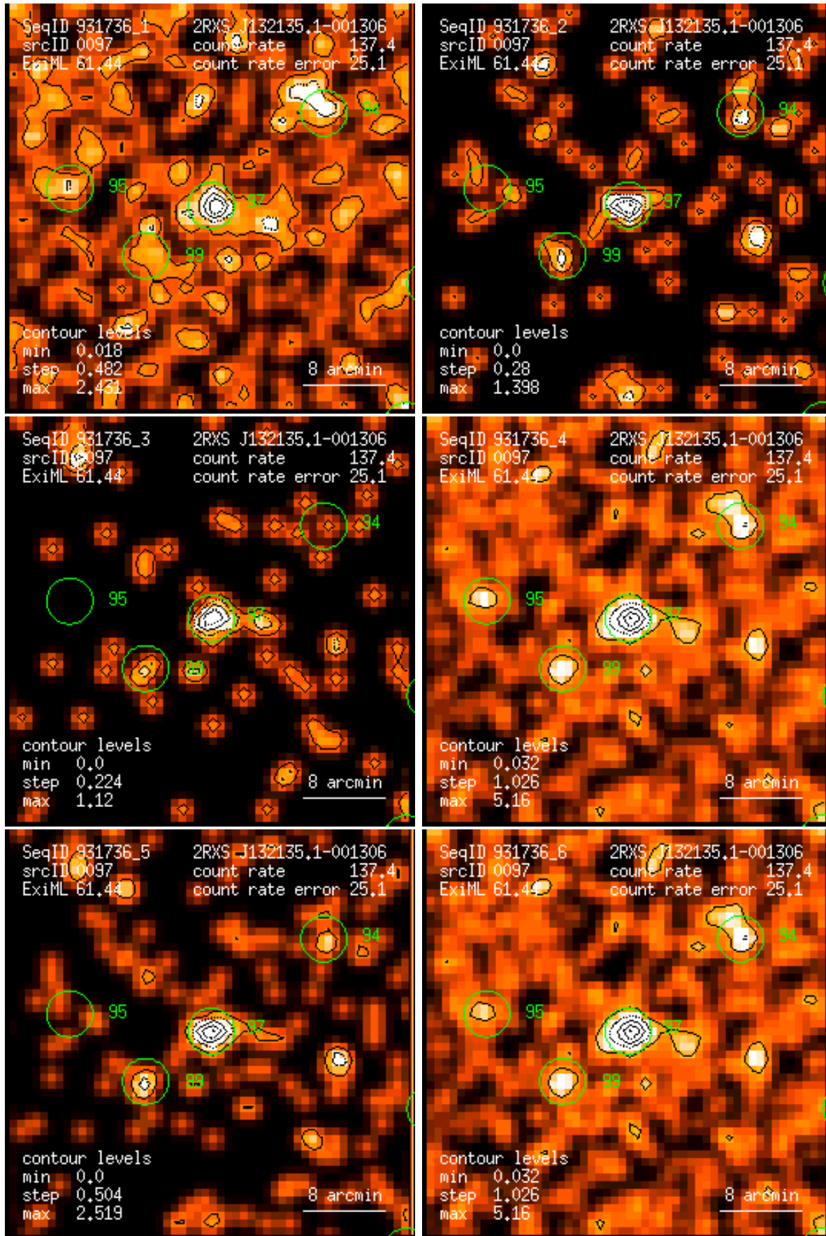
Figure 97: RASS 931736: detection 0097: band rate images, Gaussian filter: (1) PSPC channels 11 – 41, (2) 52 – 90, (3) 91 – 201, (4) 11 – 235, (5) 52 – 201, (6) 11 – 201. Broad band rates in counts/ks. Band rate contour levels in counts/ks/arcmin 2 .
