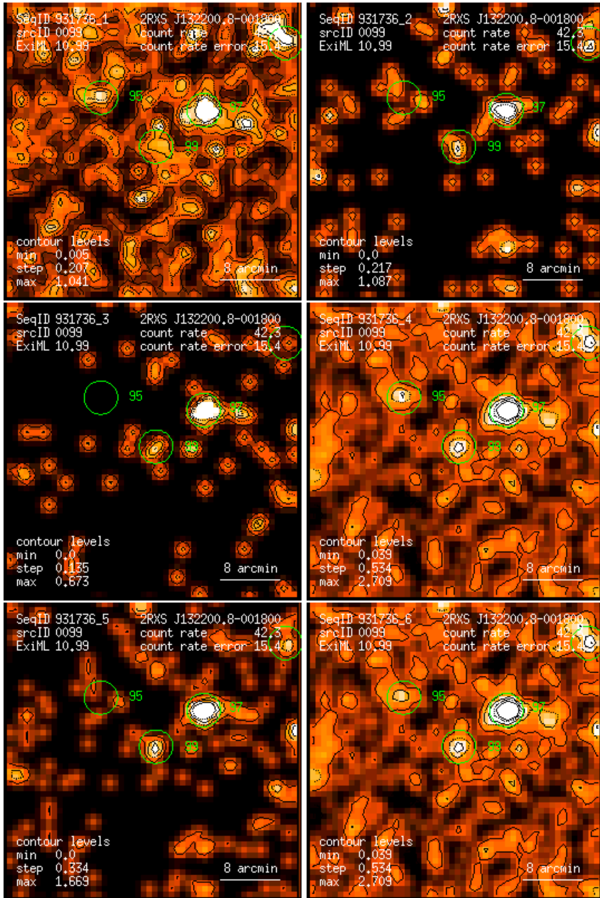
Figure 99: RASS 931736: detection 0099: band rate images, Gaussian filter: (1) PSPC channels 11 – 41, (2) 52 – 90, (3) 91 – 201, (4) 11 – 235, (5) 52 – 201, (6) 11 – 201. Broad band rates in counts/ks. Band rate contour levels in counts/ks/arcmin 2 .
