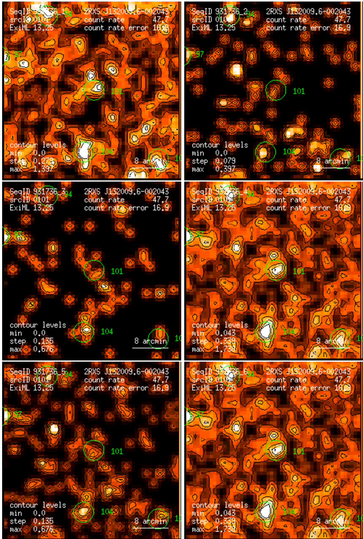
Figure 101: RASS 931736: detection 0101: band rate images, Gaussian filter: (1) PSPC channels 11 – 41, (2) 52 – 90, (3) 91 – 201, (4) 11 – 235, (5) 52 – 201, (6) 11 – 201. Broad band rates in counts/ks. Band rate contour levels in counts/ks/arcmin 2 .
