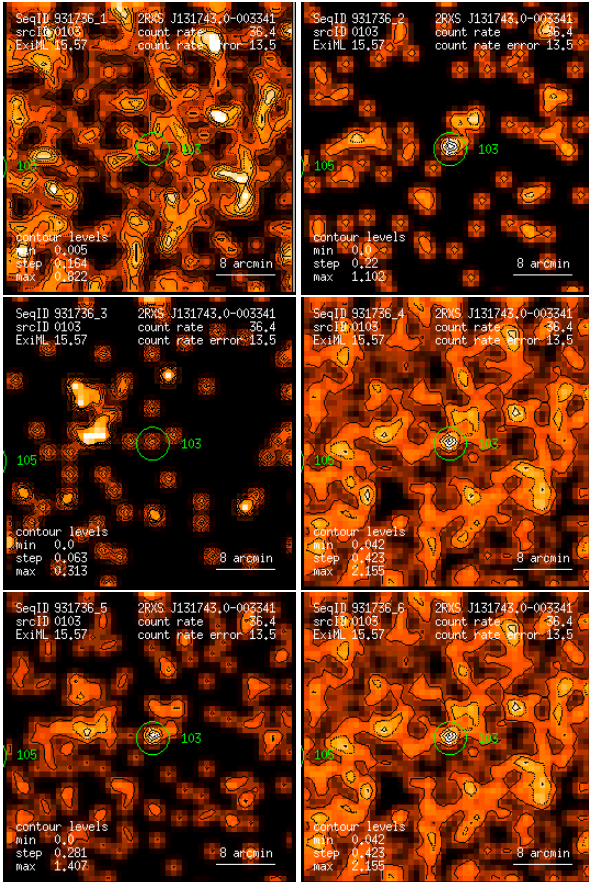
Figure 103: RASS 931736: detection 0103: band rate images, Gaussian filter: (1) PSPC channels 11 – 41, (2) 52 – 90, (3) 91 – 201, (4) 11 – 235, (5) 52 – 201, (6) 11 – 201. Broad band rates in counts/ks. Band rate contour levels in counts/ks/arcmin 2 .
