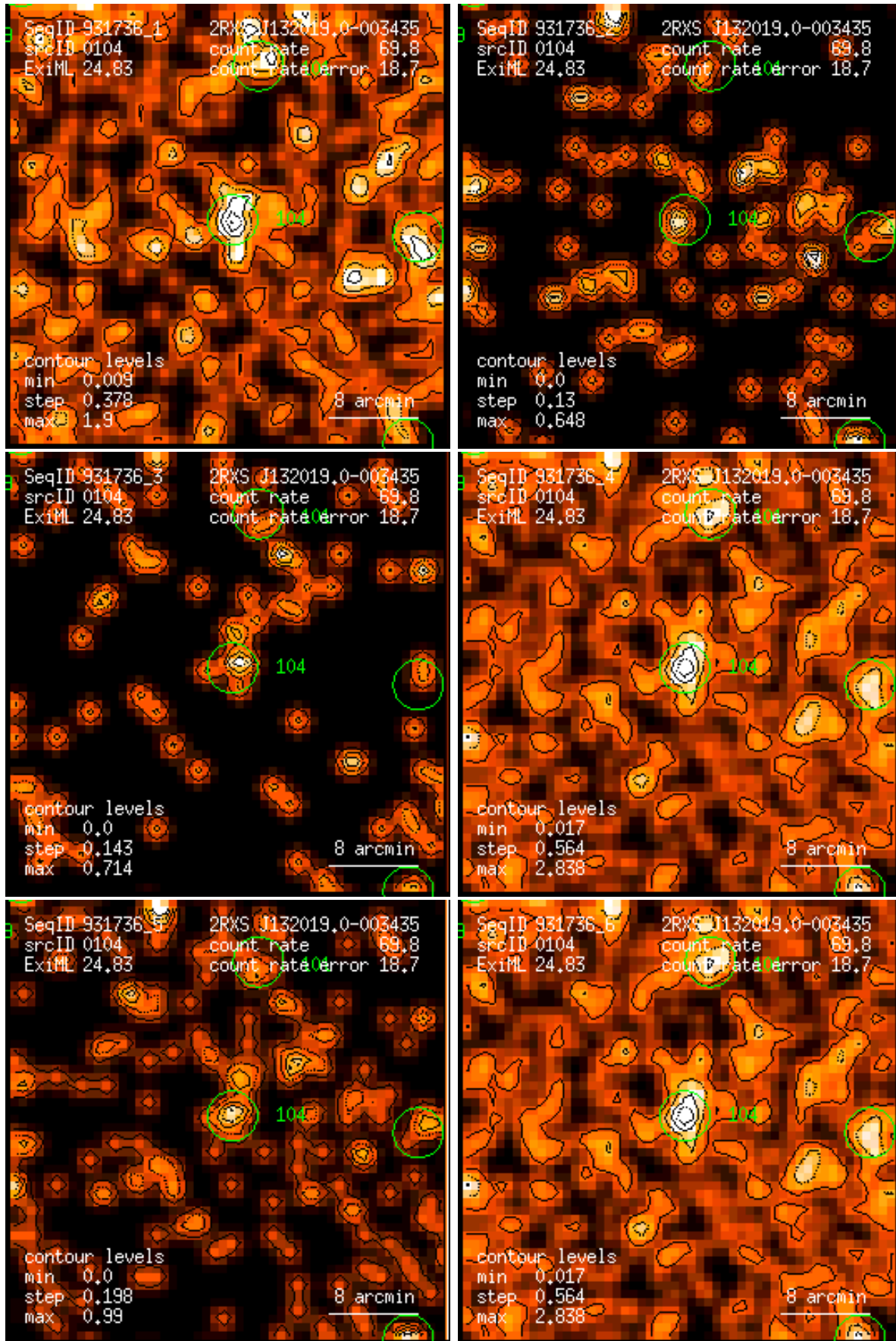
Figure 104: RASS 931736: detection 0104: band rate images, Gaussian filter: (1) PSPC channels 11 – 41, (2) 52 – 90, (3) 91 – 201, (4) 11 – 235, (5) 52 – 201, (6) 11 – 201. Broad band rates in counts/ks. Band rate contour levels in counts/ks/arcmin 2 .
