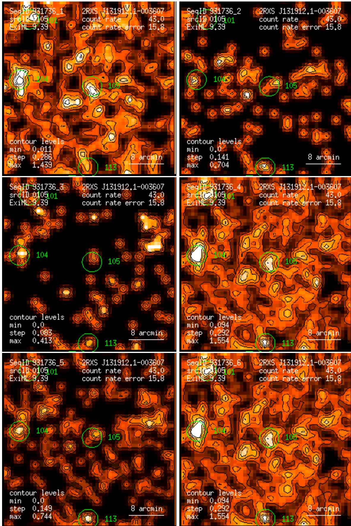
Figure 105: RASS 931736: detection 0105: band rate images, Gaussian filter: (1) PSPC channels 11 – 41, (2) 52 – 90, (3) 91 – 201, (4) 11 – 235, (5) 52 – 201, (6) 11 – 201. Broad band rates in counts/ks. Band rate contour levels in counts/ks/arcmin 2 .
