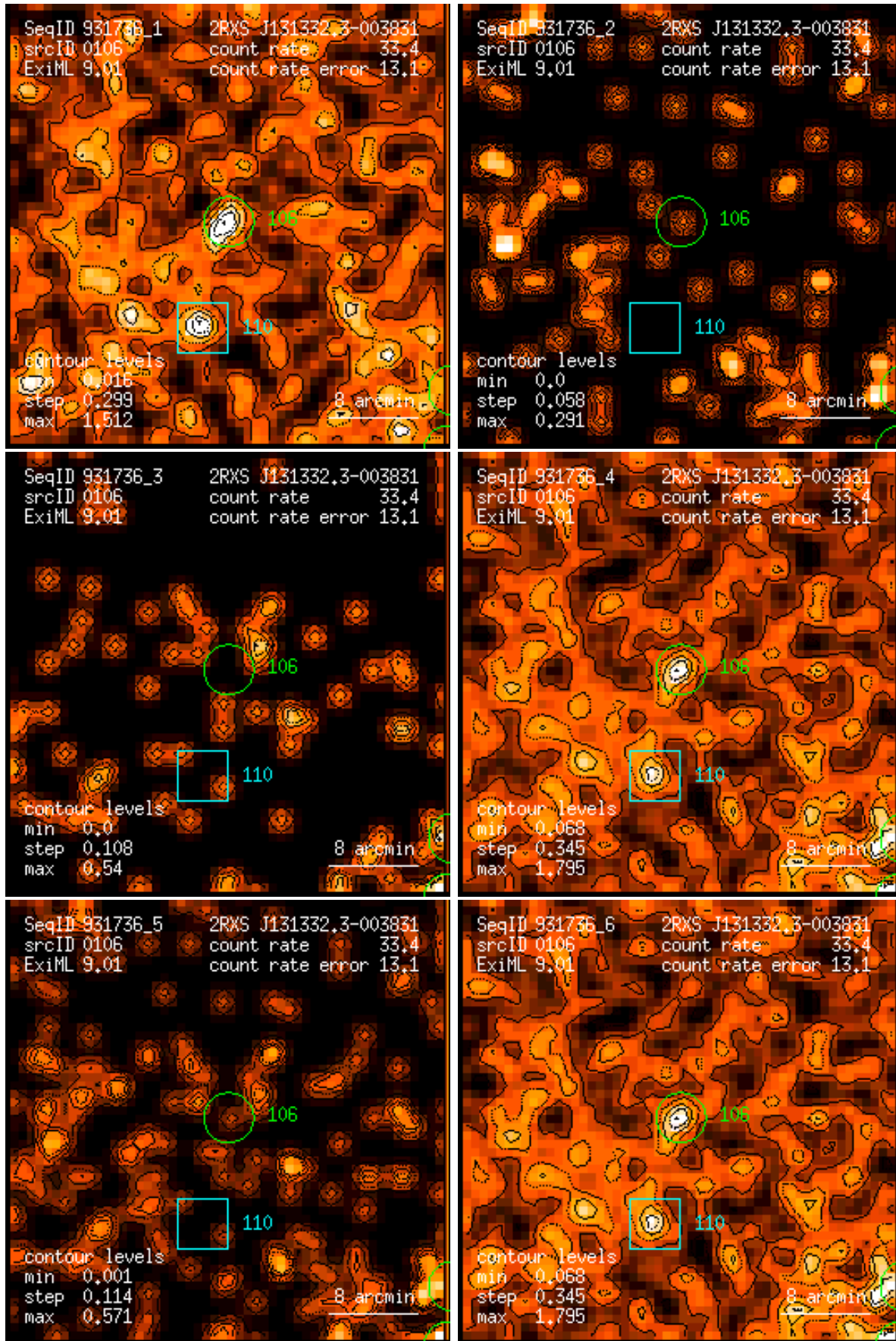
Figure 106: RASS 931736: detection 0106: band rate images, Gaussian filter: (1) PSPC channels 11 – 41, (2) 52 – 90, (3) 91 – 201, (4) 11 – 235, (5) 52 – 201, (6) 11 – 201. Broad band rates in counts/ks. Band rate contour levels in counts/ks/arcmin 2 .
