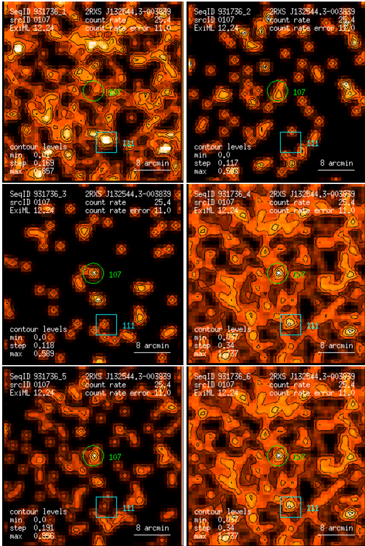
Figure 107: RASS 931736: detection 0107: band rate images, Gaussian filter: (1) PSPC channels 11 – 41, (2) 52 – 90, (3) 91 – 201, (4) 11 – 235, (5) 52 – 201, (6) 11 – 201. Broad band rates in counts/ks. Band rate contour levels in counts/ks/arcmin 2 .
