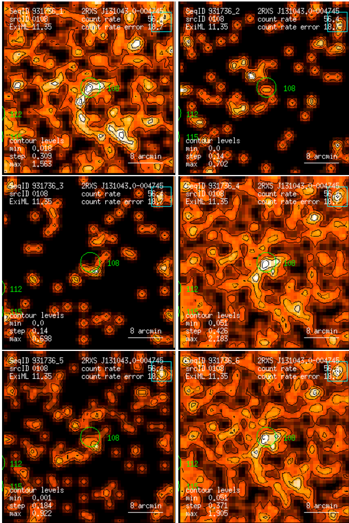
Figure 108: RASS 931736: detection 0108: band rate images, Gaussian filter: (1) PSPC channels 11 – 41, (2) 52 – 90, (3) 91 – 201, (4) 11 – 235, (5) 52 – 201, (6) 11 – 201. Broad band rates in counts/ks. Band rate contour levels in counts/ks/arcmin 2 .
