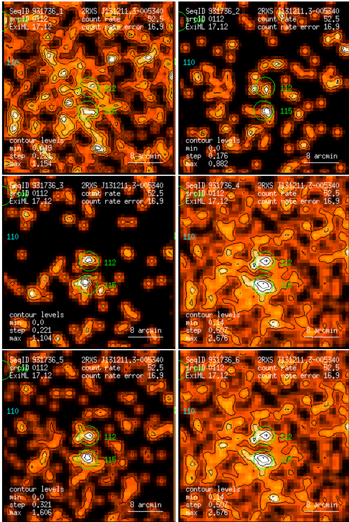
Figure 112: RASS 931736: detection 0112: band rate images, Gaussian filter: (1) PSPC channels 11 – 41, (2) 52 – 90, (3) 91 – 201, (4) 11 – 235, (5) 52 – 201, (6) 11 – 201. Broad band rates in counts/ks. Band rate contour levels in counts/ks/arcmin 2 .
