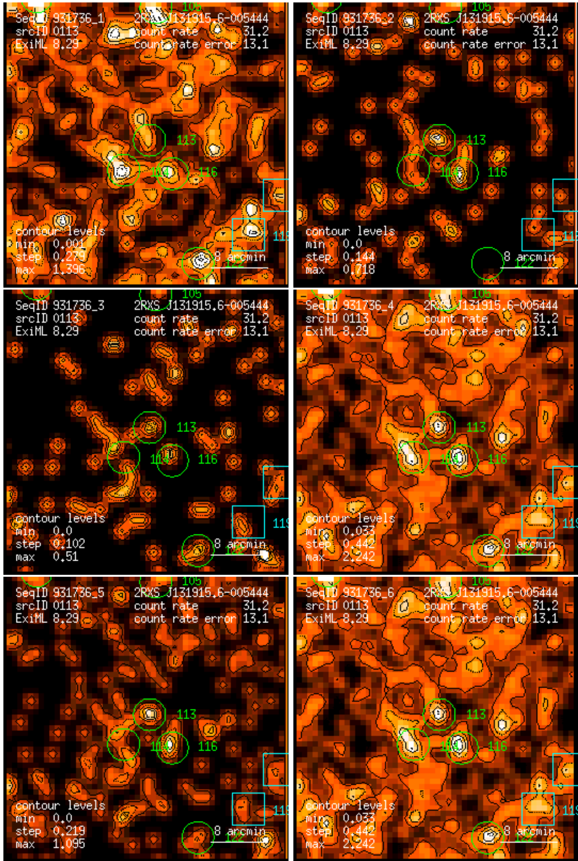
Figure 113: RASS 931736: detection 0113: band rate images, Gaussian filter: (1) PSPC channels 11 – 41, (2) 52 – 90, (3) 91 – 201, (4) 11 – 235, (5) 52 – 201, (6) 11 – 201. Broad band rates in counts/ks. Band rate contour levels in counts/ks/arcmin 2 .
