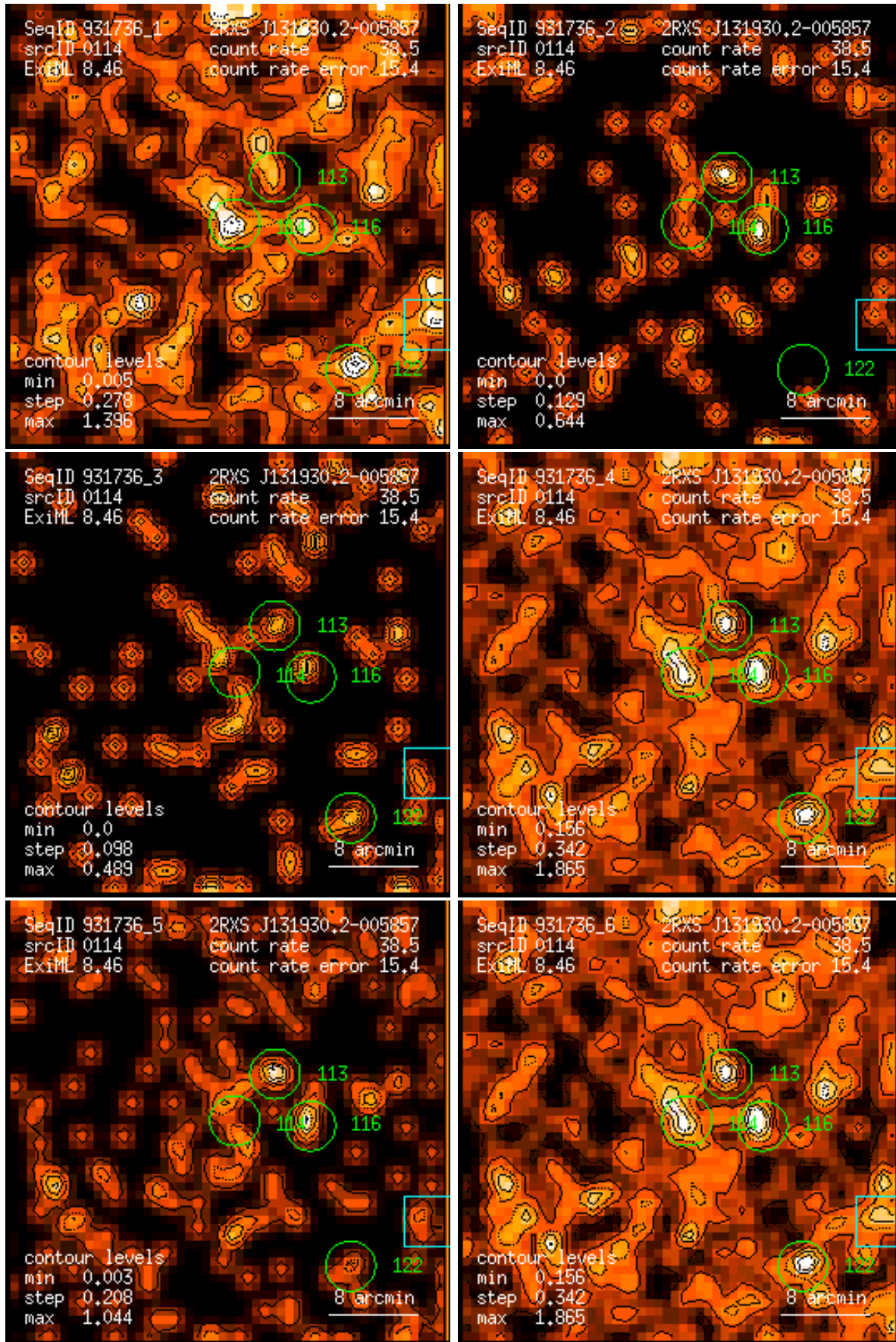
Figure 114: RASS 931736: detection 0114: band rate images, Gaussian filter: (1) PSPC channels 11 – 41, (2) 52 – 90, (3) 91 – 201, (4) 11 – 235, (5) 52 – 201, (6) 11 – 201. Broad band rates in counts/ks. Band rate contour levels in counts/ks/arcmin 2 .
