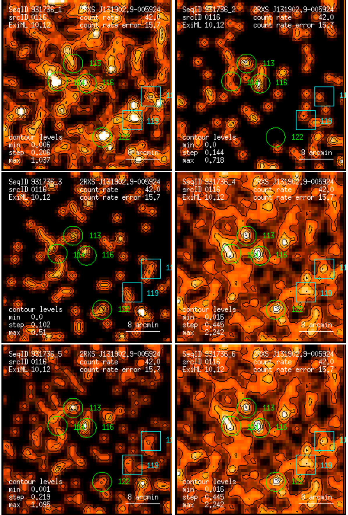
Figure 116: RASS 931736: detection 0116: band rate images, Gaussian filter: (1) PSPC channels 11 – 41, (2) 52 – 90, (3) 91 – 201, (4) 11 – 235, (5) 52 – 201, (6) 11 – 201. Broad band rates in counts/ks. Band rate contour levels in counts/ks/arcmin 2 .
