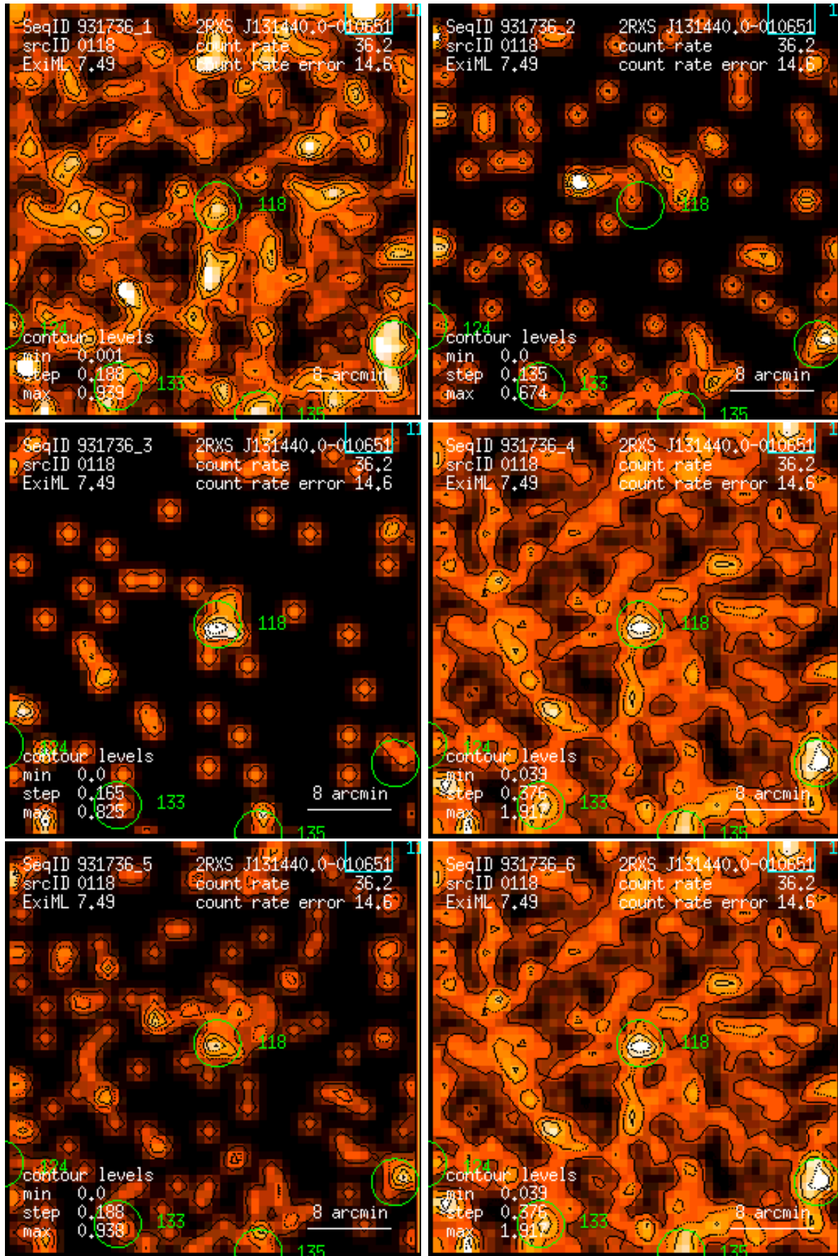
Figure 118: RASS 931736: detection 0118: band rate images, Gaussian filter: (1) PSPC channels 11 – 41, (2) 52 – 90, (3) 91 – 201, (4) 11 – 235, (5) 52 – 201, (6) 11 – 201. Broad band rates in counts/ks. Band rate contour levels in counts/ks/arcmin 2 .
