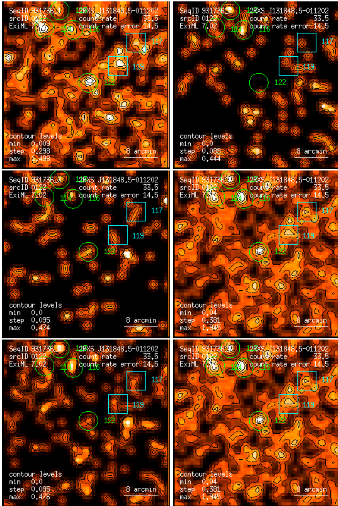
Figure 122: RASS 931736: detection 0122: band rate images, Gaussian filter: (1) PSPC channels 11 – 41, (2) 52 – 90, (3) 91 – 201, (4) 11 – 235, (5) 52 – 201, (6) 11 – 201. Broad band rates in counts/ks. Band rate contour levels in counts/ks/arcmin 2 .
