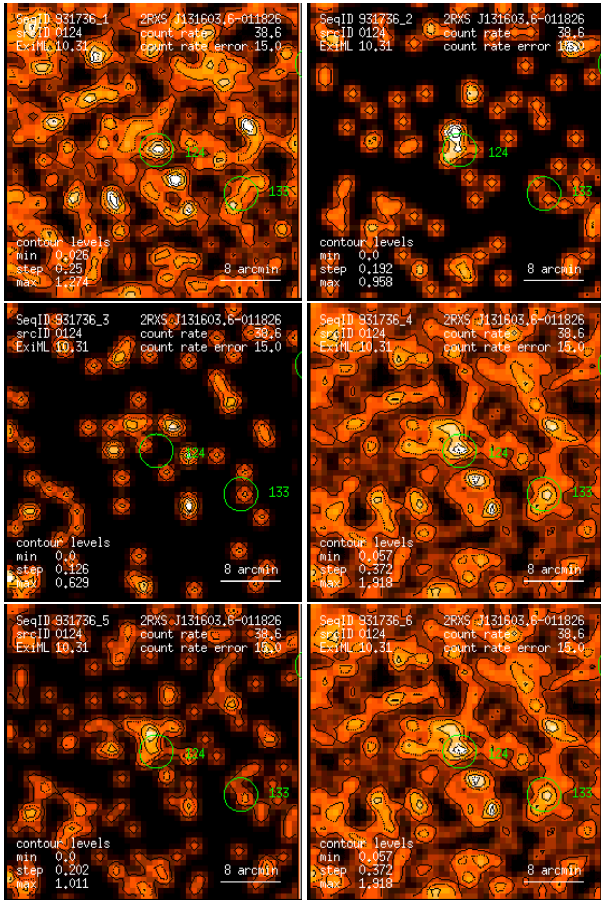
Figure 124: RASS 931736: detection 0124: band rate images, Gaussian filter: (1) PSPC channels 11 – 41, (2) 52 – 90, (3) 91 – 201, (4) 11 – 235, (5) 52 – 201, (6) 11 – 201. Broad band rates in counts/ks. Band rate contour levels in counts/ks/arcmin 2 .
