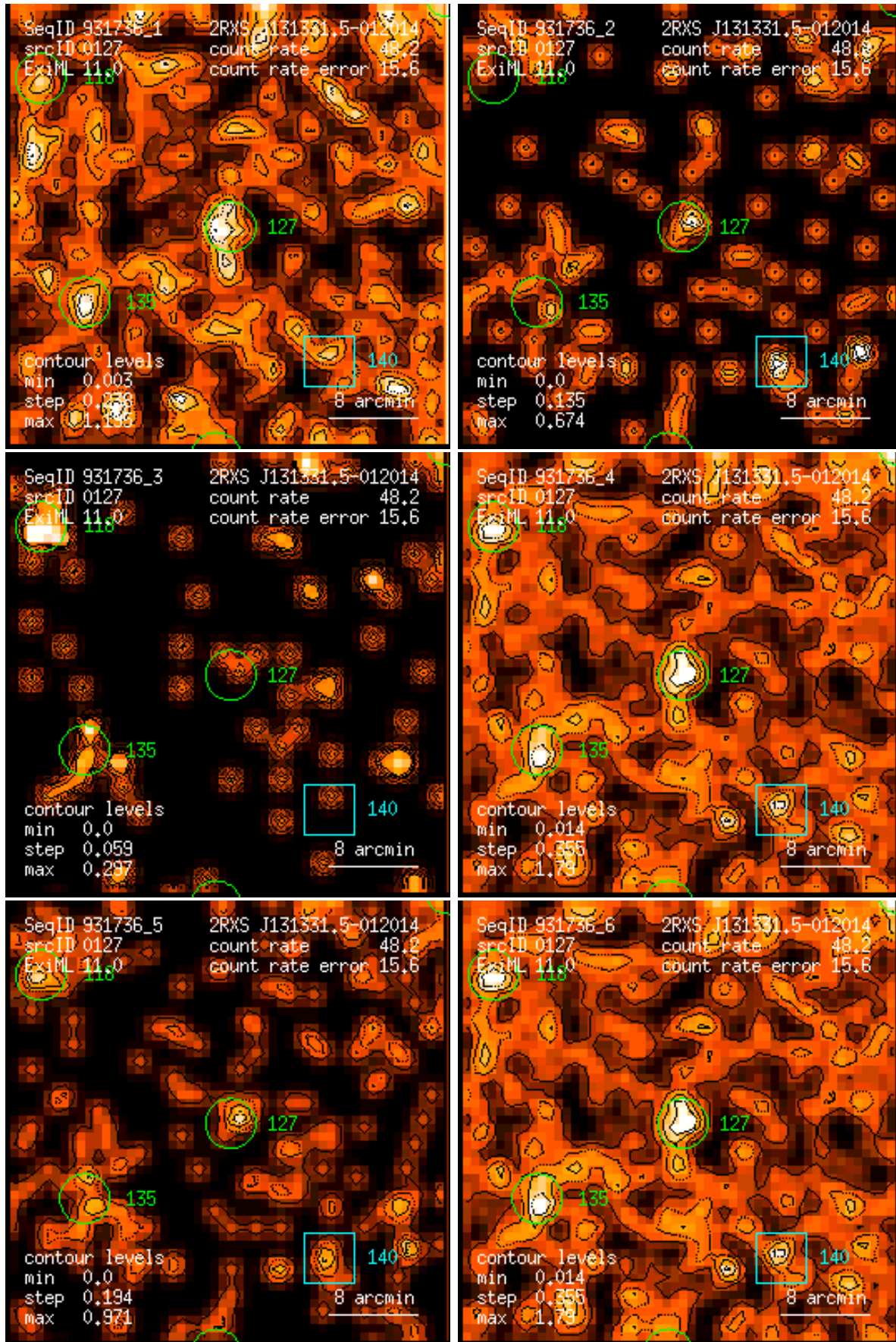
Figure 127: RASS 931736: detection 0127: band rate images, Gaussian filter: (1) PSPC channels 11 – 41, (2) 52 – 90, (3) 91 – 201, (4) 11 – 235, (5) 52 – 201, (6) 11 – 201. Broad band rates in counts/ks. Band rate contour levels in counts/ks/arcmin 2 .
