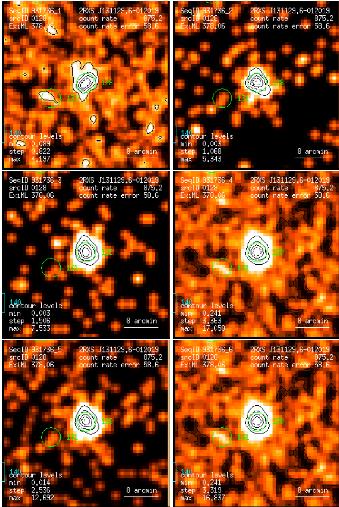
Figure 128: RASS 931736: detection 0128: band rate images, Gaussian filter: (1) PSPC channels 11 – 41, (2) 52 – 90, (3) 91 – 201, (4) 11 – 235, (5) 52 – 201, (6) 11 – 201. Broad band rates in counts/ks. Band rate contour levels in counts/ks/arcmin 2 .
