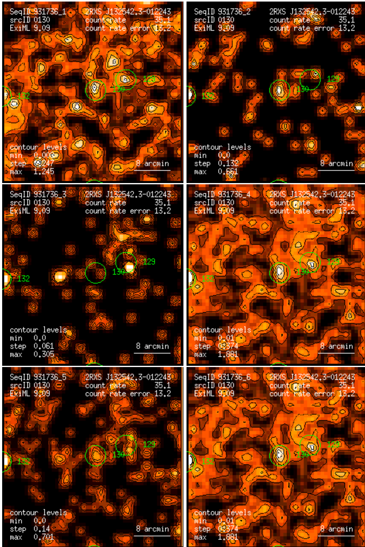
Figure 130: RASS 931736: detection 0130: band rate images, Gaussian filter: (1) PSPC channels 11 – 41, (2) 52 – 90, (3) 91 – 201, (4) 11 – 235, (5) 52 – 201, (6) 11 – 201. Broad band rates in counts/ks. Band rate contour levels in counts/ks/arcmin 2 .
