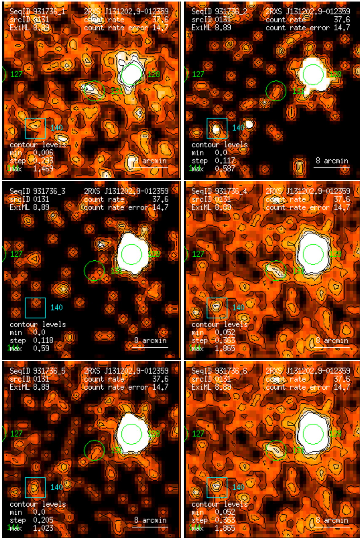
Figure 131: RASS 931736: detection 0131: band rate images, Gaussian filter: (1) PSPC channels 11 – 41, (2) 52 – 90, (3) 91 – 201, (4) 11 – 235, (5) 52 – 201, (6) 11 – 201. Broad band rates in counts/ks. Band rate contour levels in counts/ks/arcmin 2 .
