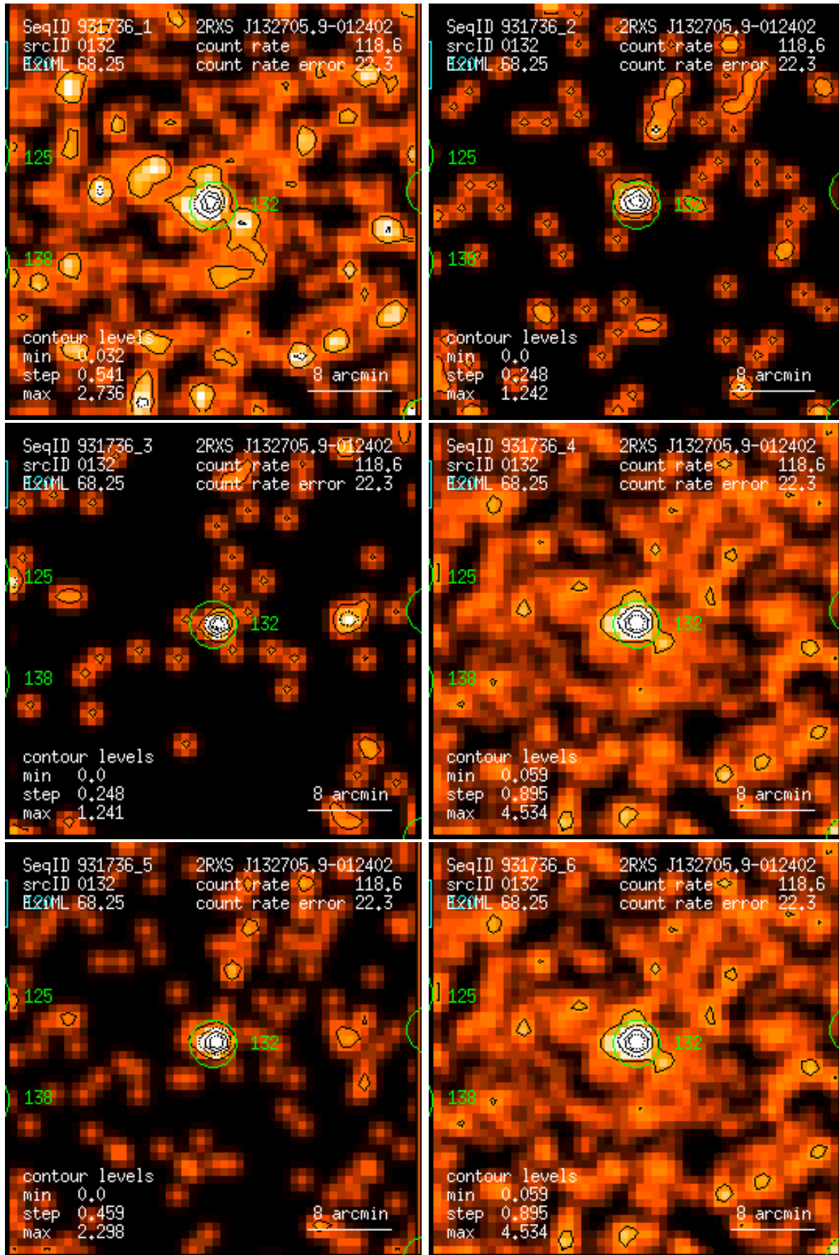
Figure 132: RASS 931736: detection 0132: band rate images, Gaussian filter: (1) PSPC channels 11 – 41, (2) 52 – 90, (3) 91 – 201, (4) 11 – 235, (5) 52 – 201, (6) 11 – 201. Broad band rates in counts/ks. Band rate contour levels in counts/ks/arcmin 2 .
