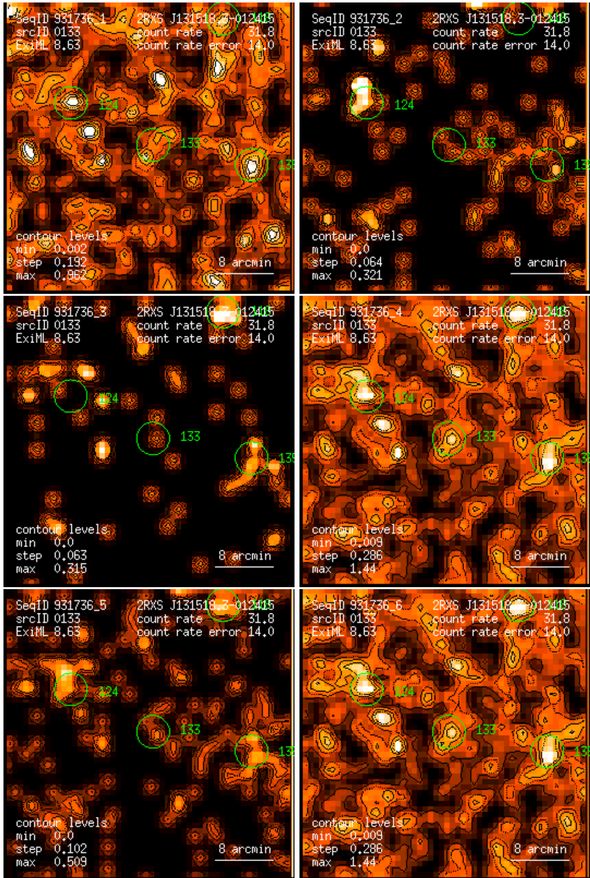
Figure 133: RASS 931736: detection 0133: band rate images, Gaussian filter: (1) PSPC channels 11 – 41, (2) 52 – 90, (3) 91 – 201, (4) 11 – 235, (5) 52 – 201, (6) 11 – 201. Broad band rates in counts/ks. Band rate contour levels in counts/ks/arcmin 2 .
