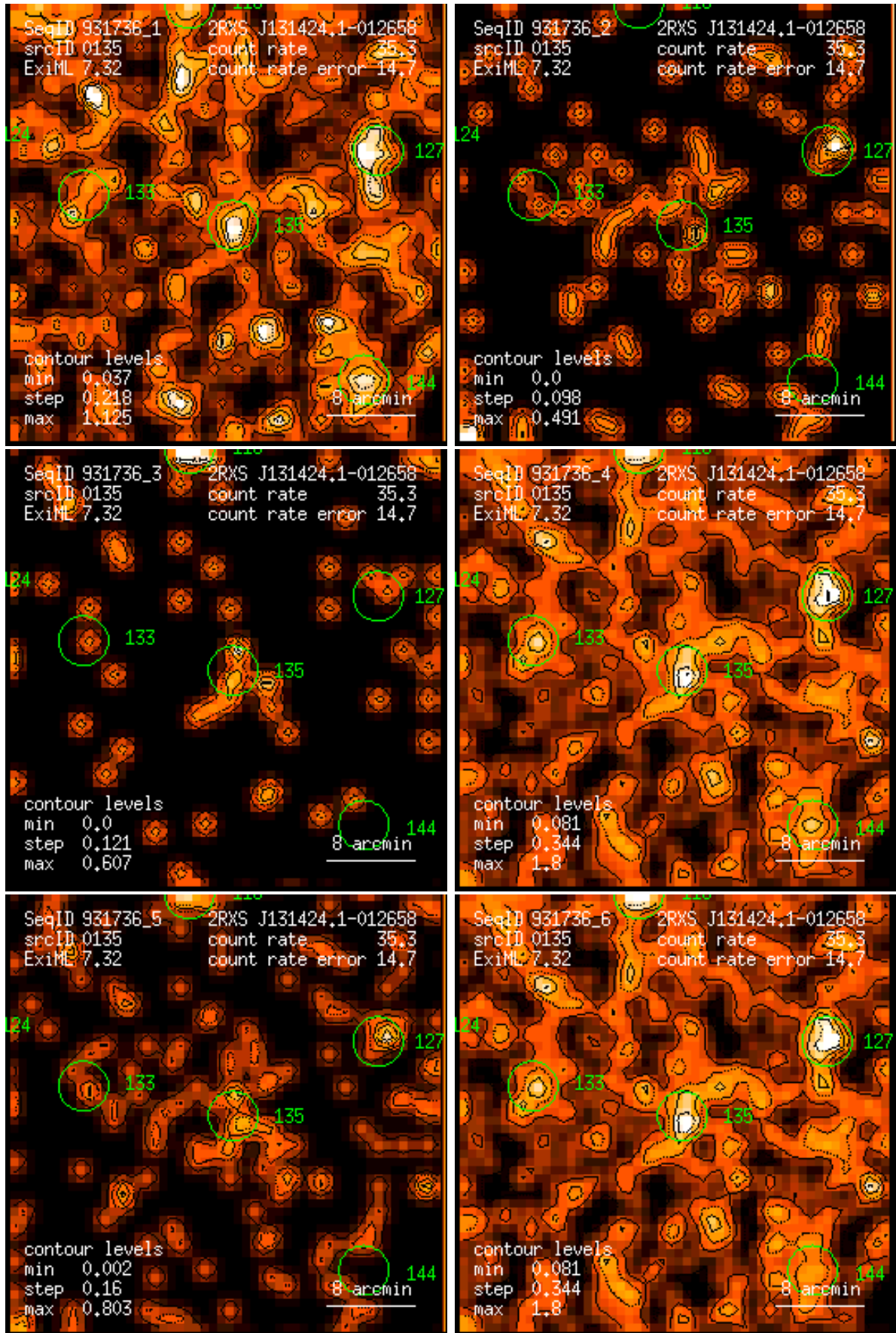
Figure 135: RASS 931736: detection 0135: band rate images, Gaussian filter: (1) PSPC channels 11 – 41, (2) 52 – 90, (3) 91 – 201, (4) 11 – 235, (5) 52 – 201, (6) 11 – 201. Broad band rates in counts/ks. Band rate contour levels in counts/ks/arcmin 2 .
