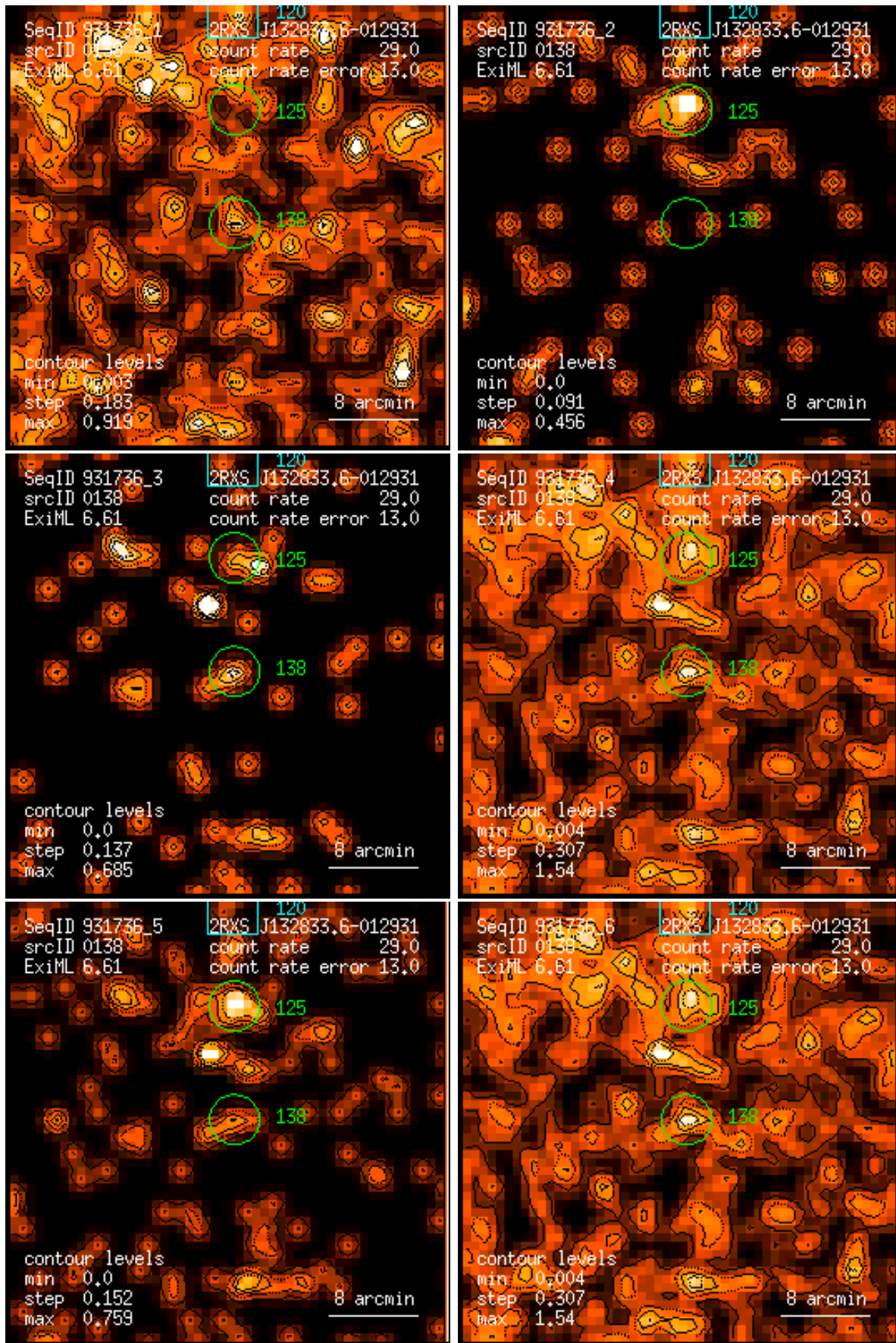
Figure 138: RASS 931736: detection 0138: band rate images, Gaussian filter: (1) PSPC channels 11 – 41, (2) 52 – 90, (3) 91 – 201, (4) 11 – 235, (5) 52 – 201, (6) 11 – 201. Broad band rates in counts/ks. Band rate contour levels in counts/ks/arcmin 2 .
