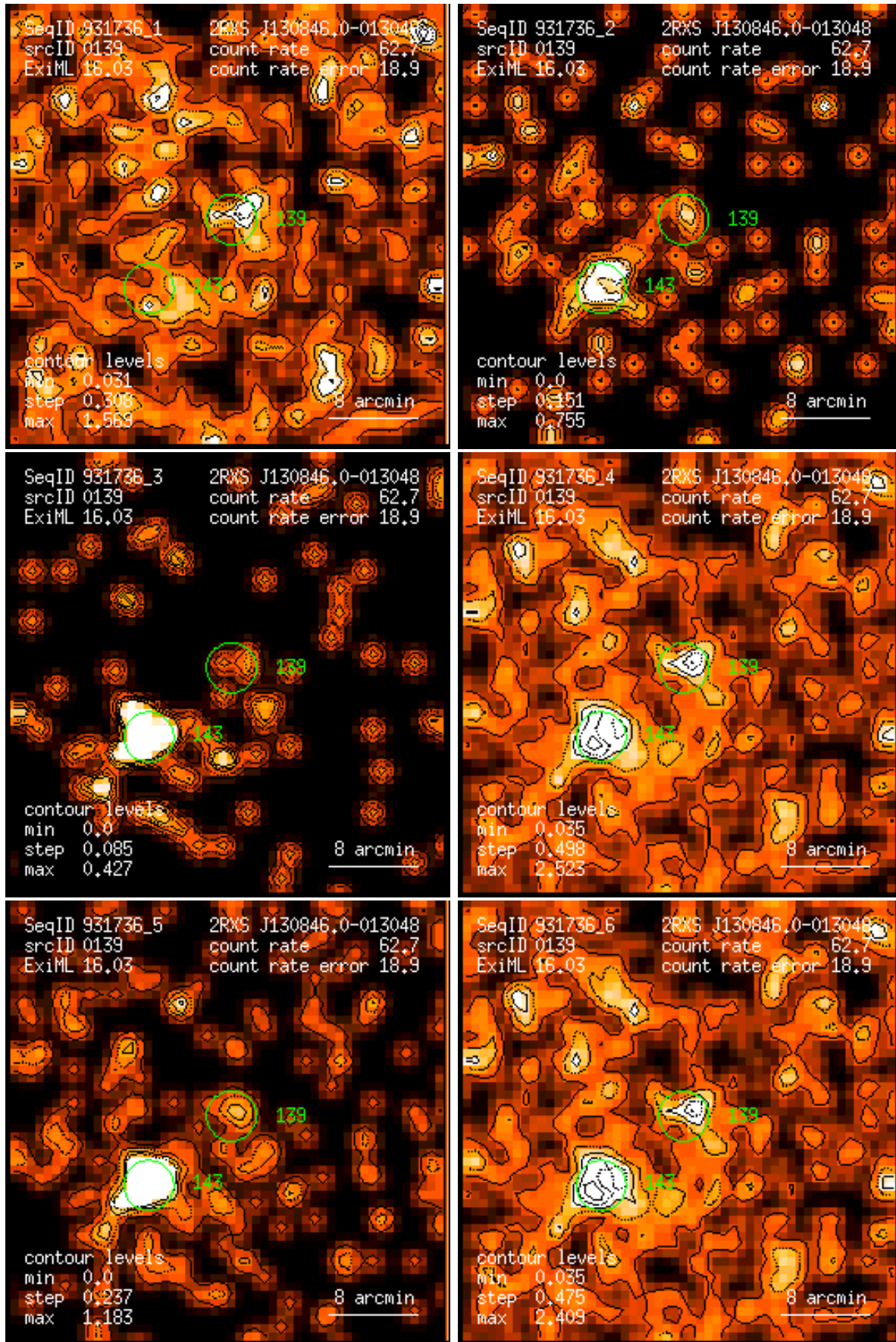
Figure 139: RASS 931736: detection 0139: band rate images, Gaussian filter: (1) PSPC channels 11 – 41, (2) 52 – 90, (3) 91 – 201, (4) 11 – 235, (5) 52 – 201, (6) 11 – 201. Broad band rates in counts/ks. Band rate contour levels in counts/ks/arcmin 2 .
