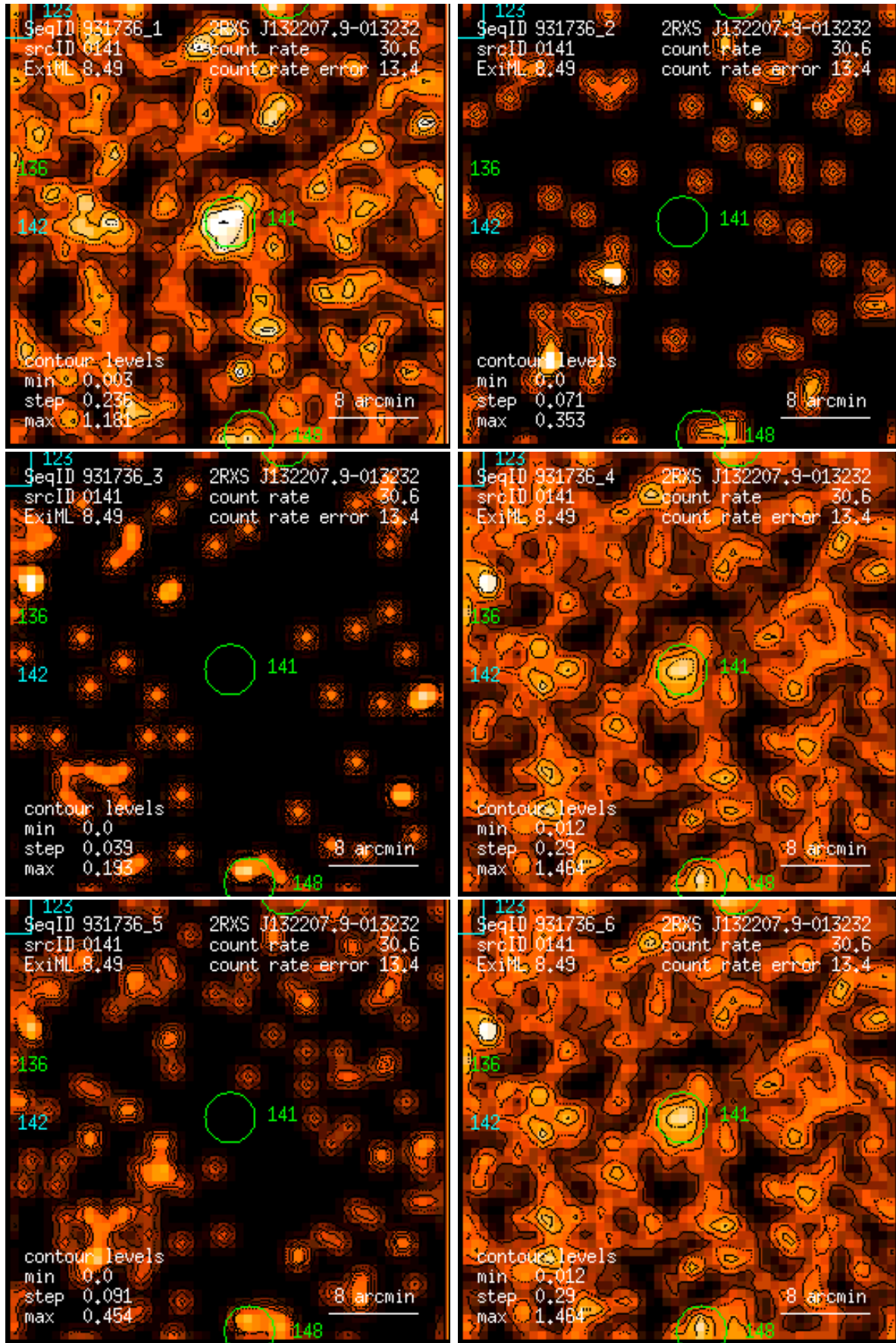
Figure 141: RASS 931736: detection 0141: band rate images, Gaussian filter: (1) PSPC channels 11 – 41, (2) 52 – 90, (3) 91 – 201, (4) 11 – 235, (5) 52 – 201, (6) 11 – 201. Broad band rates in counts/ks. Band rate contour levels in counts/ks/arcmin 2 .
