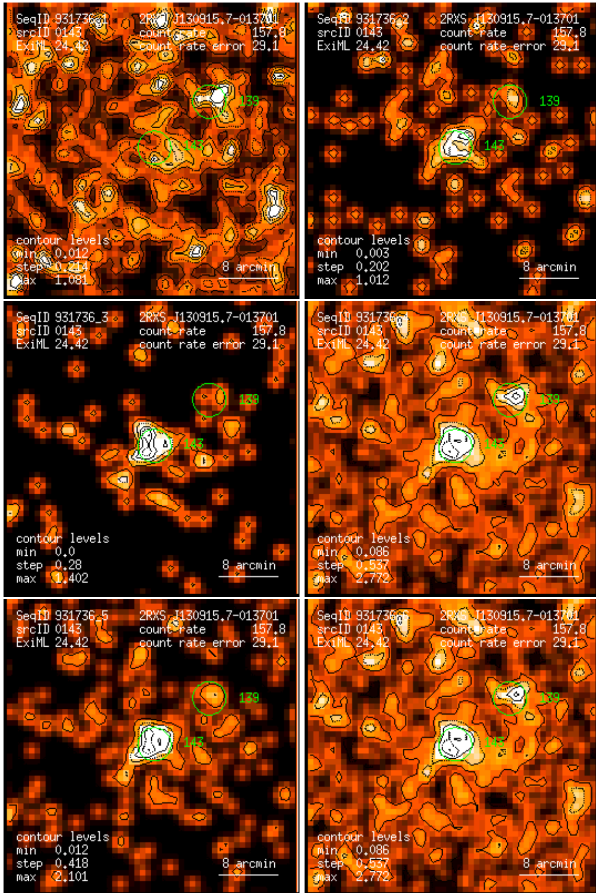
Figure 143: RASS 931736: detection 0143: band rate images, Gaussian filter: (1) PSPC channels 11 – 41, (2) 52 – 90, (3) 91 – 201, (4) 11 – 235, (5) 52 – 201, (6) 11 – 201. Broad band rates in counts/ks. Band rate contour levels in counts/ks/arcmin 2 .
