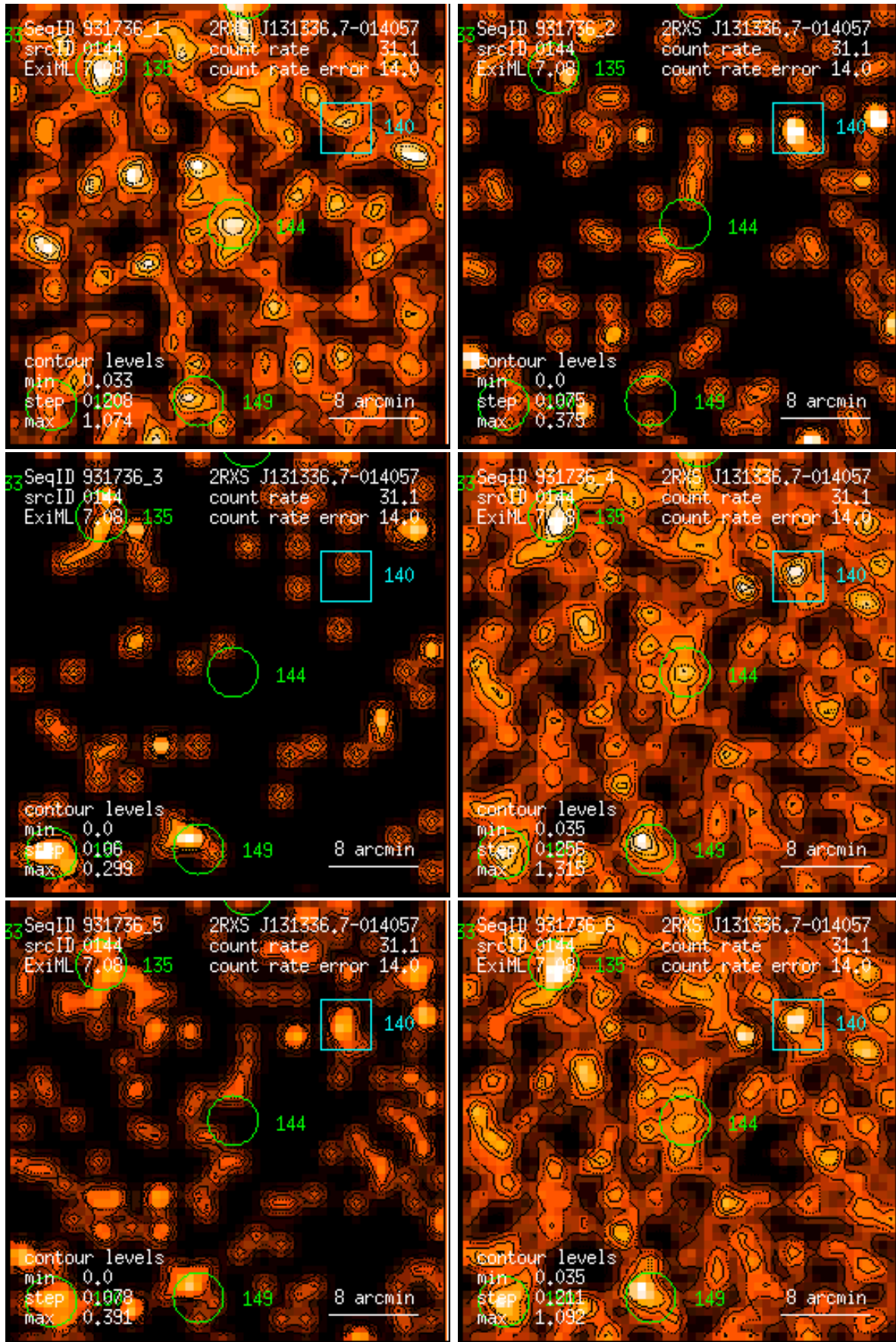
Figure 144: RASS 931736: detection 0144: band rate images, Gaussian filter: (1) PSPC channels 11 – 41, (2) 52 – 90, (3) 91 – 201, (4) 11 – 235, (5) 52 – 201, (6) 11 – 201. Broad band rates in counts/ks. Band rate contour levels in counts/ks/arcmin 2 .
