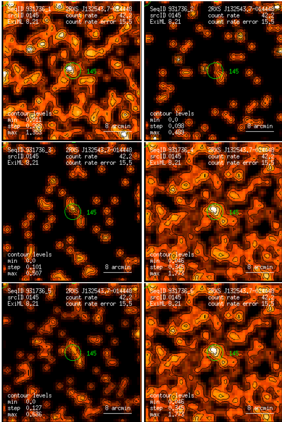
Figure 145: RASS 931736: detection 0145: band rate images, Gaussian filter: (1) PSPC channels 11 – 41, (2) 52 – 90, (3) 91 – 201, (4) 11 – 235, (5) 52 – 201, (6) 11 – 201. Broad band rates in counts/ks. Band rate contour levels in counts/ks/arcmin 2 .
