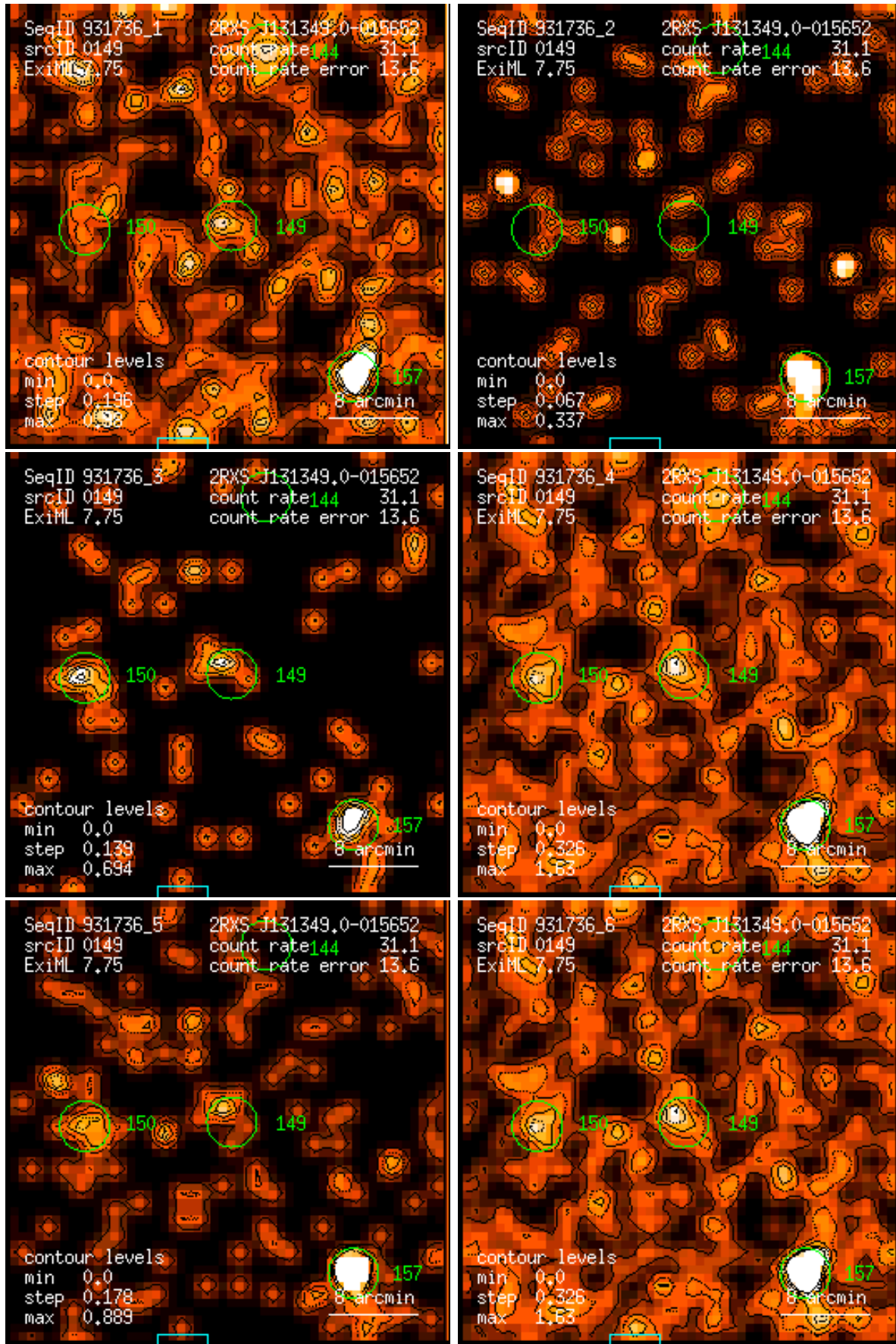
Figure 149: RASS 931736: detection 0149: band rate images, Gaussian filter: (1) PSPC channels 11 – 41, (2) 52 – 90, (3) 91 – 201, (4) 11 – 235, (5) 52 – 201, (6) 11 – 201. Broad band rates in counts/ks. Band rate contour levels in counts/ks/arcmin 2 .
