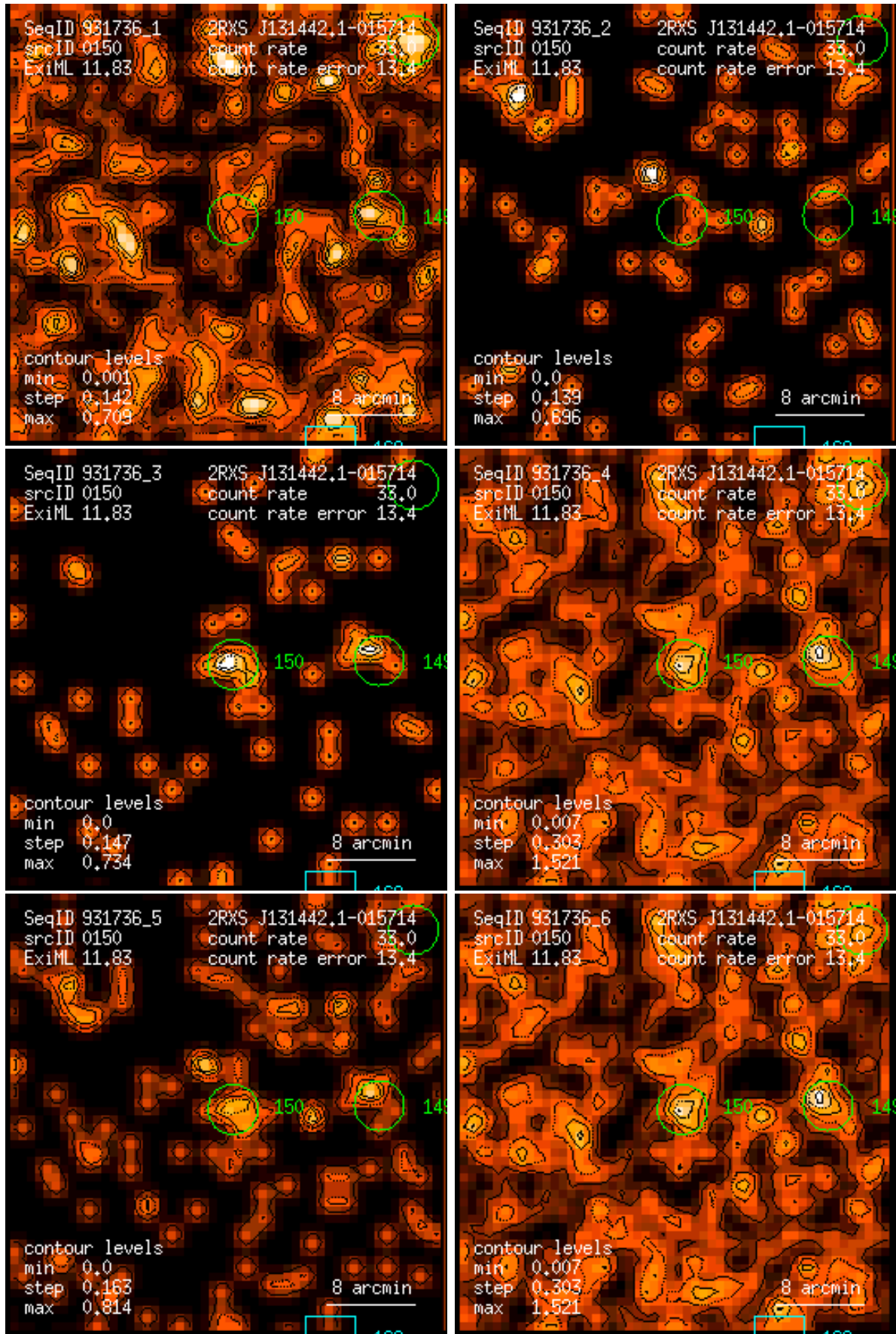
Figure 150: RASS 931736: detection 0150: band rate images, Gaussian filter: (1) PSPC channels 11 – 41, (2) 52 – 90, (3) 91 – 201, (4) 11 – 235, (5) 52 – 201, (6) 11 – 201. Broad band rates in counts/ks. Band rate contour levels in counts/ks/arcmin 2 .
