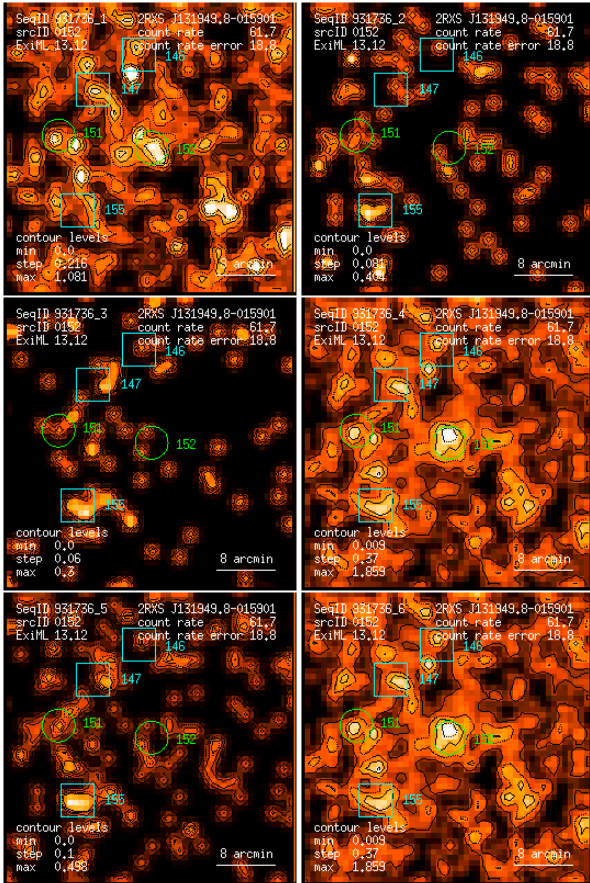
Figure 152: RASS 931736: detection 0152: band rate images, Gaussian filter: (1) PSPC channels 11 – 41, (2) 52 – 90, (3) 91 – 201, (4) 11 – 235, (5) 52 – 201, (6) 11 – 201. Broad band rates in counts/ks. Band rate contour levels in counts/ks/arcmin 2 .
