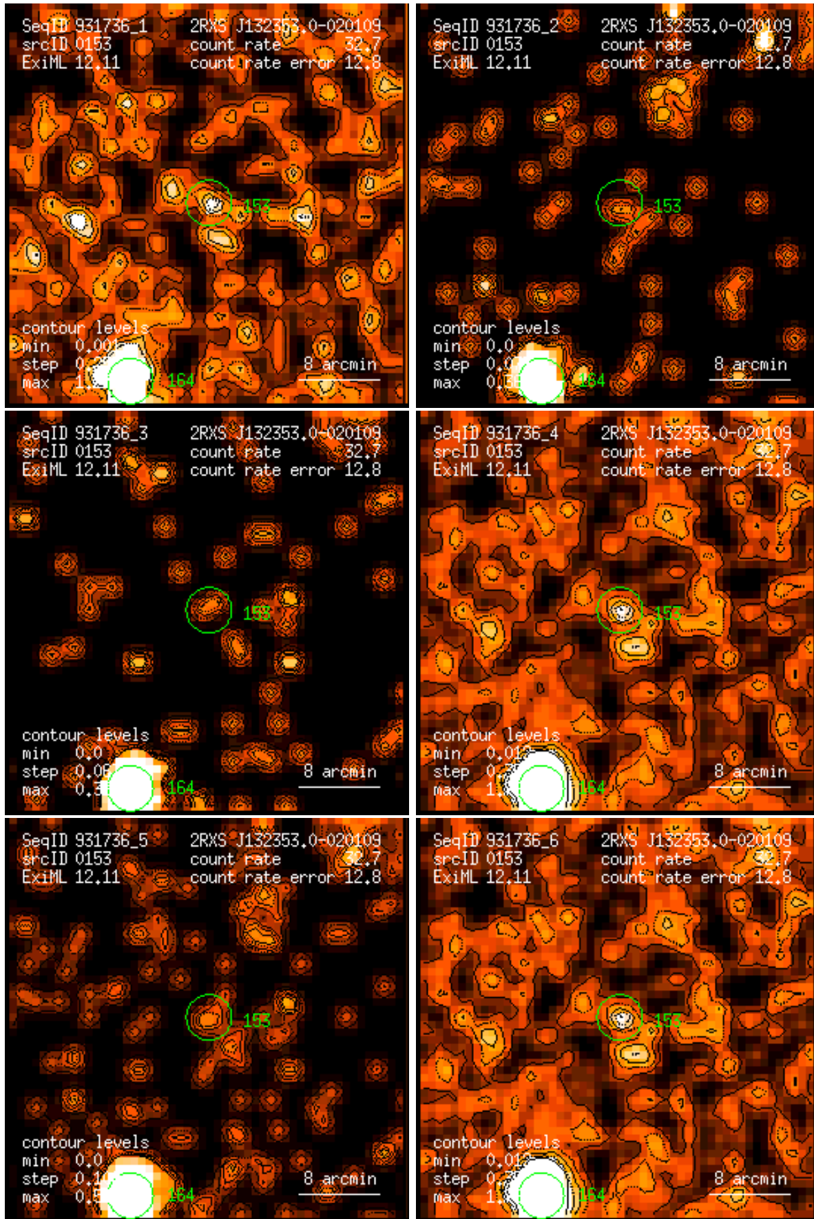
Figure 153: RASS 931736: detection 0153: band rate images, Gaussian filter: (1) PSPC channels 11 – 41, (2) 52 – 90, (3) 91 – 201, (4) 11 – 235, (5) 52 – 201, (6) 11 – 201. Broad band rates in counts/ks. Band rate contour levels in counts/ks/arcmin 2 .
