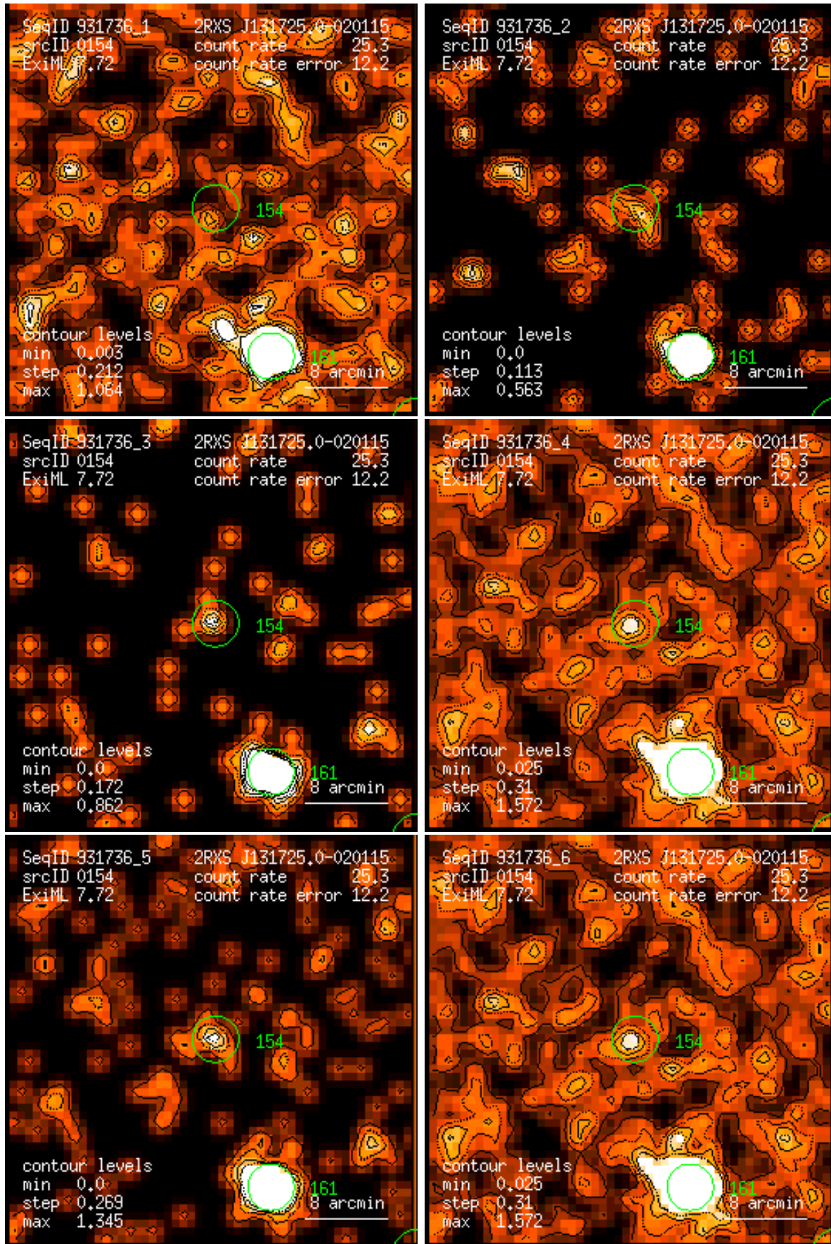
Figure 154: RASS 931736: detection 0154: band rate images, Gaussian filter: (1) PSPC channels 11 – 41, (2) 52 – 90, (3) 91 – 201, (4) 11 – 235, (5) 52 – 201, (6) 11 – 201. Broad band rates in counts/ks. Band rate contour levels in counts/ks/arcmin 2 .
