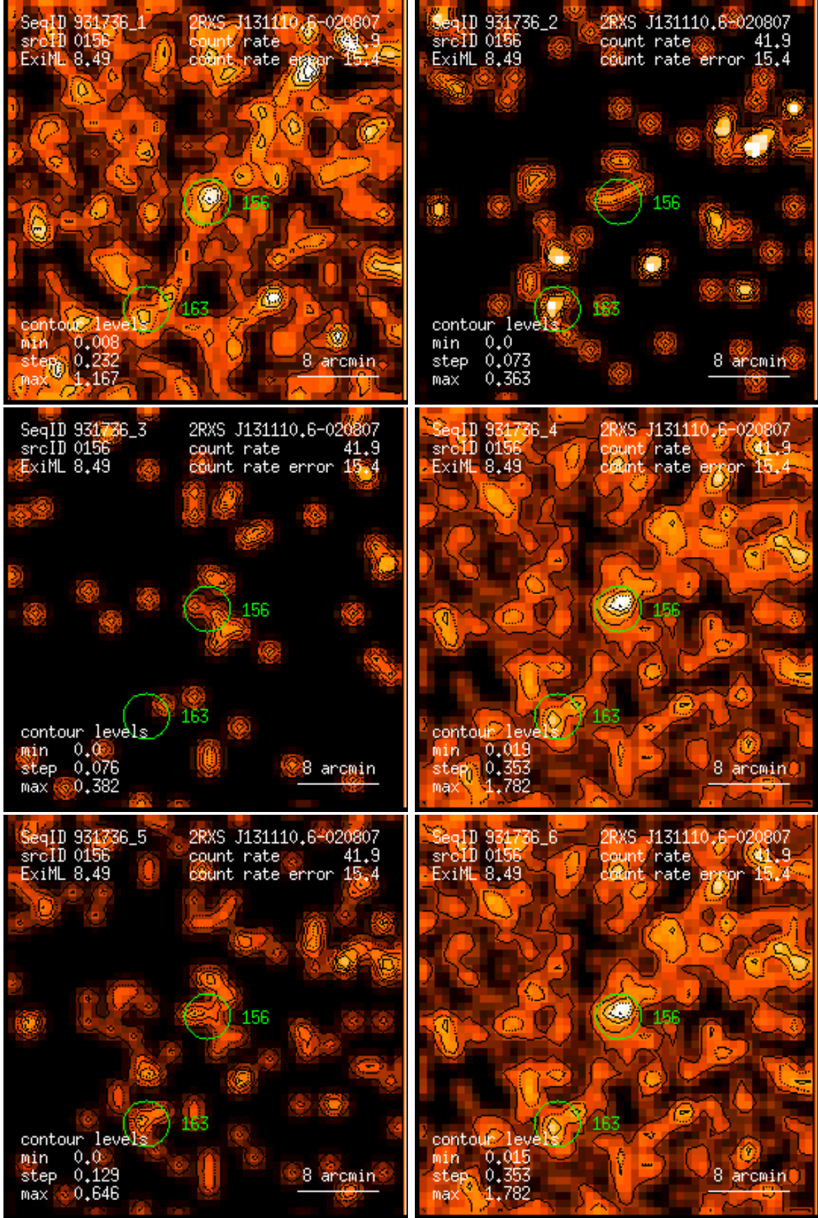
Figure 156: RASS 931736: detection 0156: band rate images, Gaussian filter: (1) PSPC channels 11 – 41, (2) 52 – 90, (3) 91 – 201, (4) 11 – 235, (5) 52 – 201, (6) 11 – 201. Broad band rates in counts/ks. Band rate contour levels in counts/ks/arcmin 2 .
