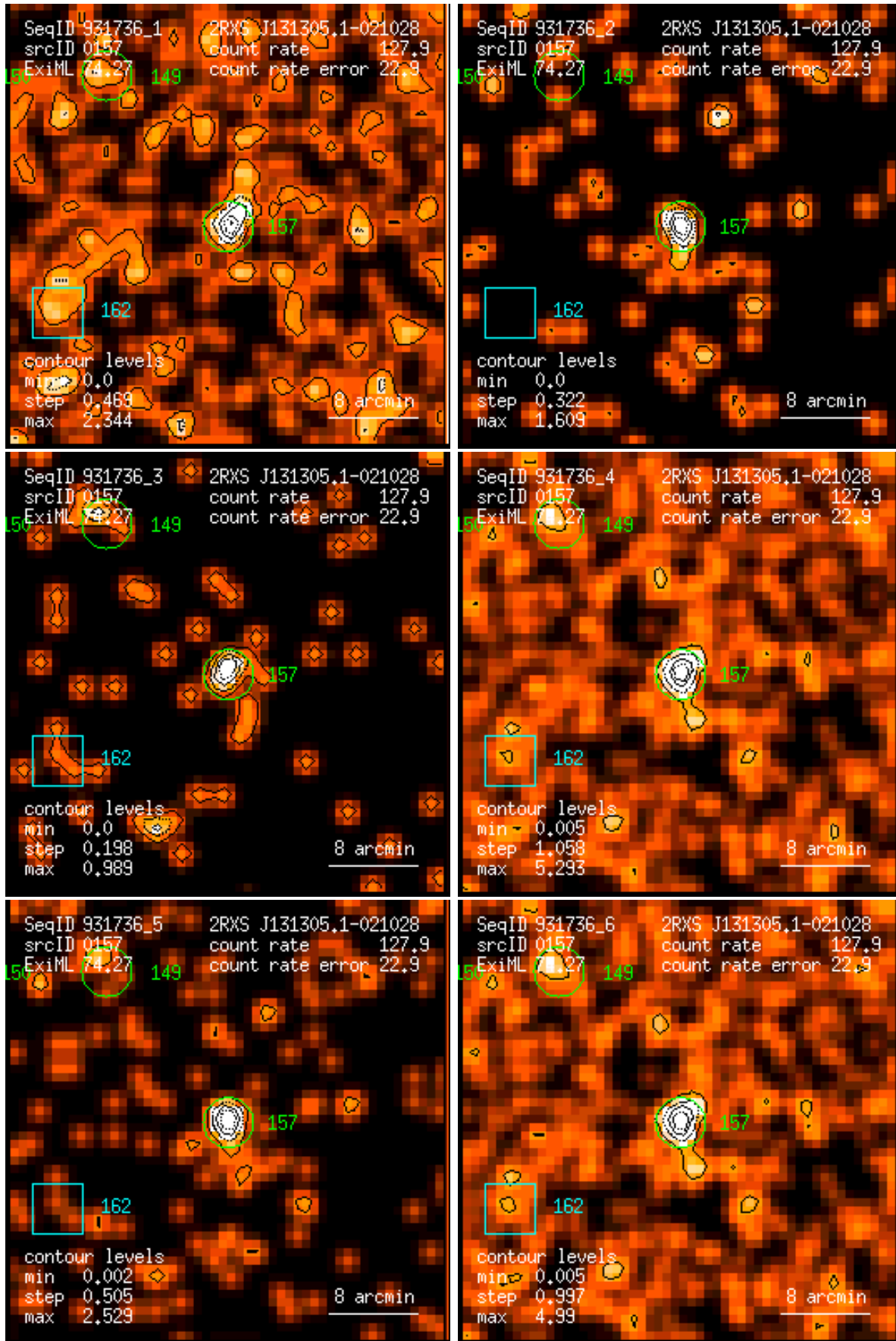
Figure 157: RASS 931736: detection 0157: band rate images, Gaussian filter: (1) PSPC channels 11 – 41, (2) 52 – 90, (3) 91 – 201, (4) 11 – 235, (5) 52 – 201, (6) 11 – 201. Broad band rates in counts/ks. Band rate contour levels in counts/ks/arcmin 2 .
