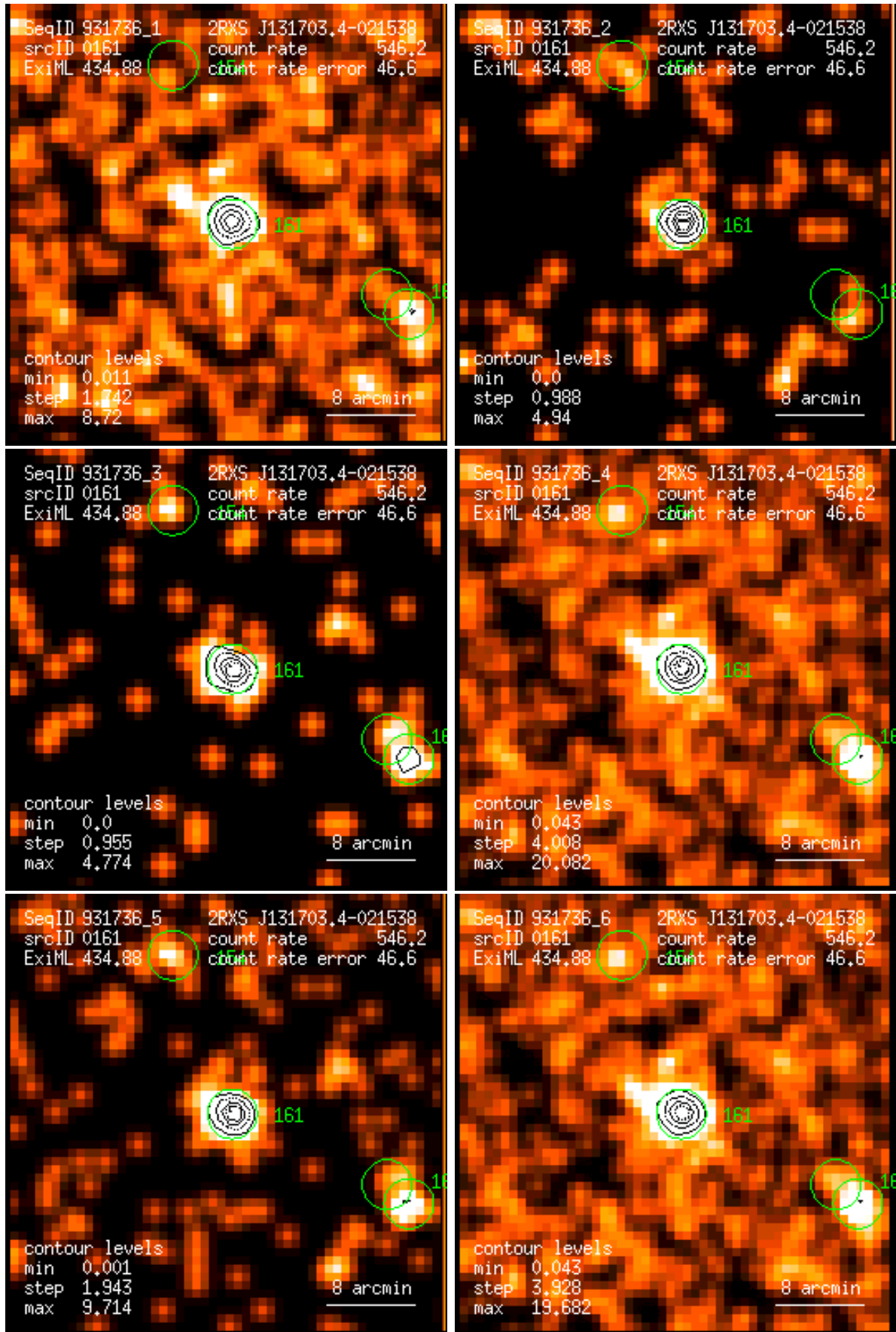
Figure 161: RASS 931736: detection 0161: band rate images, Gaussian filter: (1) PSPC channels 11 – 41, (2) 52 – 90, (3) 91 – 201, (4) 11 – 235, (5) 52 – 201, (6) 11 – 201. Broad band rates in counts/ks. Band rate contour levels in counts/ks/arcmin 2 .
