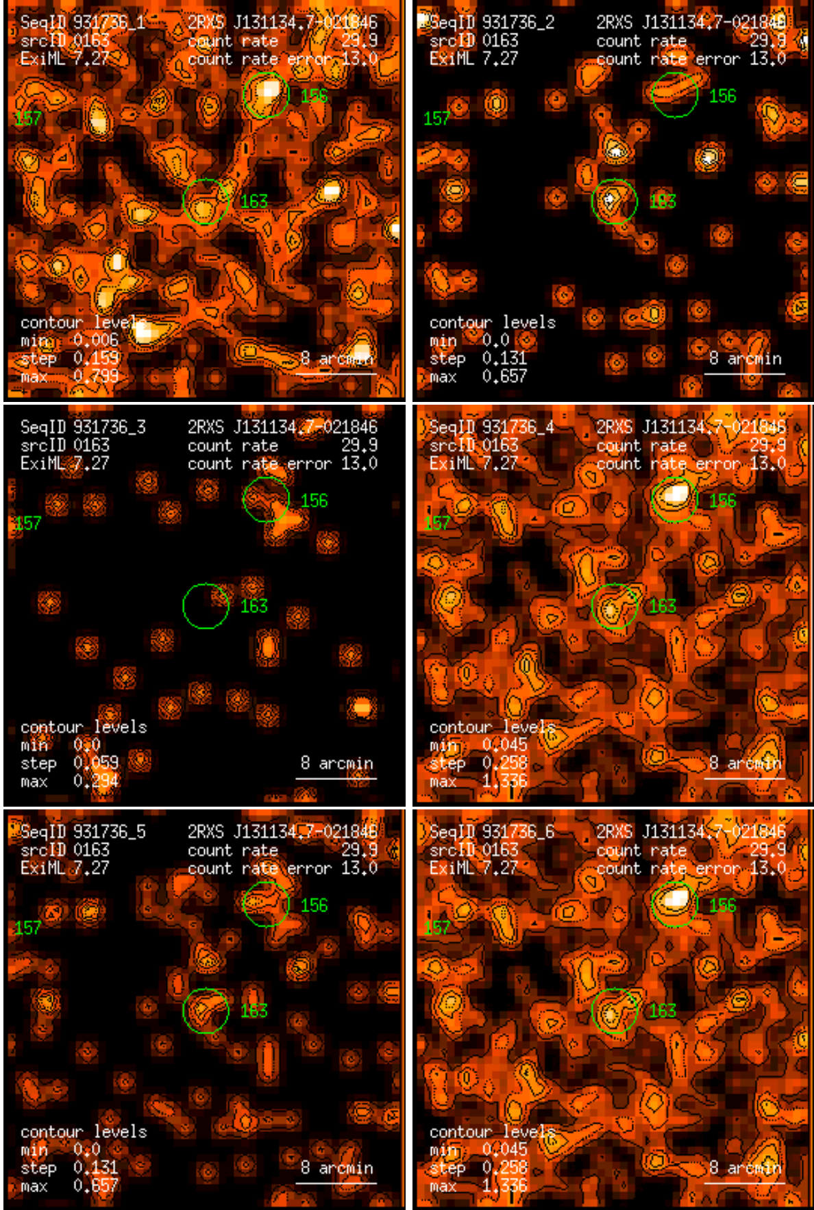
Figure 163: RASS 931736: detection 0163: band rate images, Gaussian filter: (1) PSPC channels 11 – 41, (2) 52 – 90, (3) 91 – 201, (4) 11 – 235, (5) 52 – 201, (6) 11 – 201. Broad band rates in counts/ks. Band rate contour levels in counts/ks/arcmin 2 .
