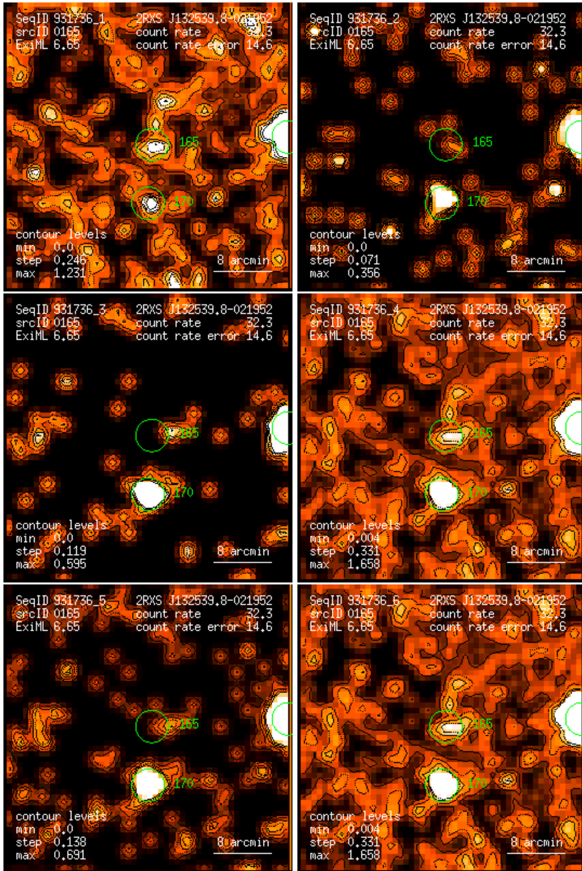
Figure 165: RASS 931736: detection 0165: band rate images, Gaussian filter: (1) PSPC channels 11 – 41, (2) 52 – 90, (3) 91 – 201, (4) 11 – 235, (5) 52 – 201, (6) 11 – 201. Broad band rates in counts/ks. Band rate contour levels in counts/ks/arcmin 2 .
