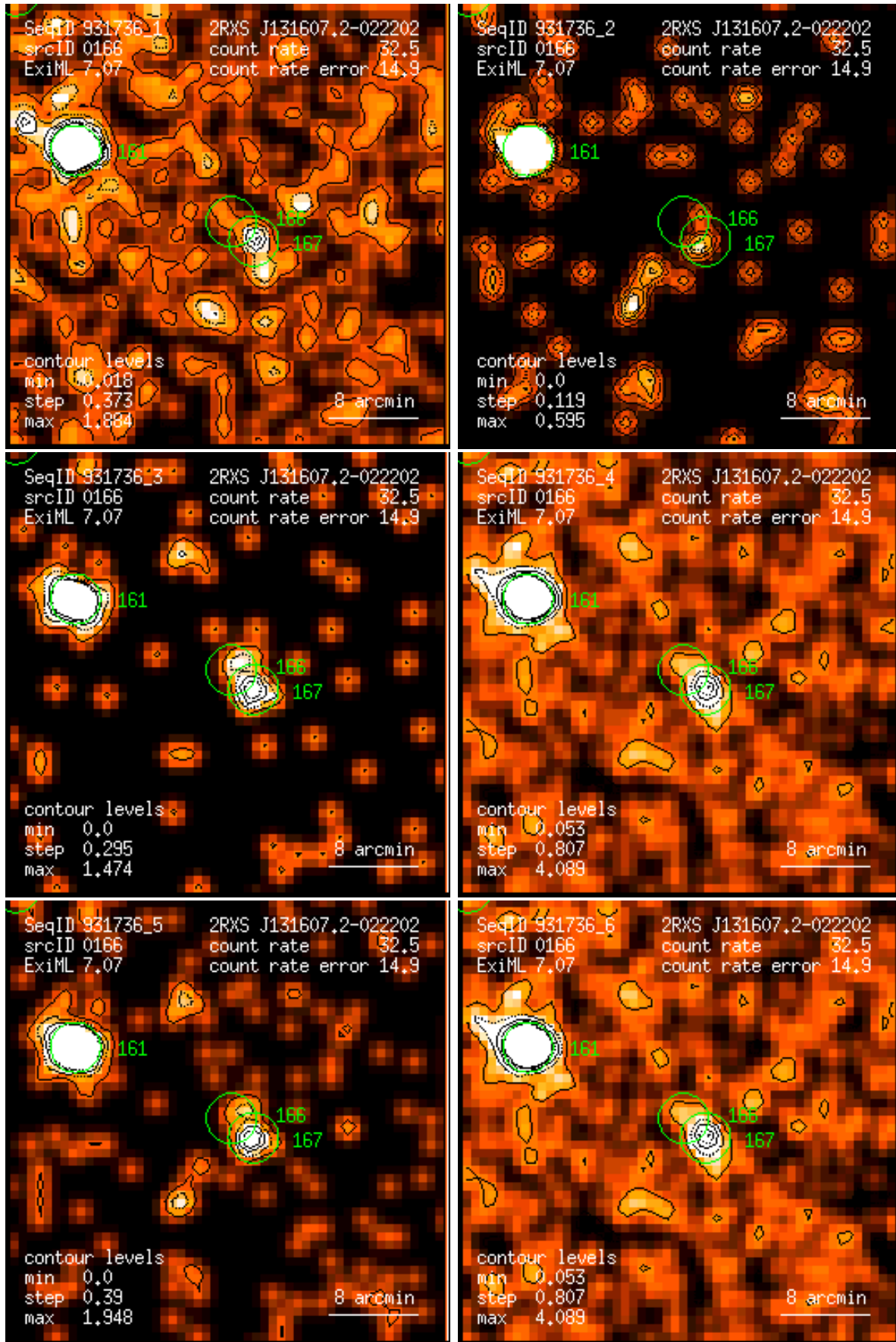
Figure 166: RASS 931736: detection 0166: band rate images, Gaussian filter: (1) PSPC channels 11 – 41, (2) 52 – 90, (3) 91 – 201, (4) 11 – 235, (5) 52 – 201, (6) 11 – 201. Broad band rates in counts/ks. Band rate contour levels in counts/ks/arcmin 2 .
